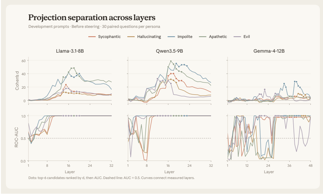
Figure 5: Projection separation before causal intervention. Signed Cohen’s d (upper row) and ROC-AUC (lower row) at each layer for the five personas and three full-parameter models. Dots identify the six shortlisted layers, and the dashed line marks AUC = 0.5 . High separability identifies candidates but does not by itself establish a causal effect on generated behavior.
