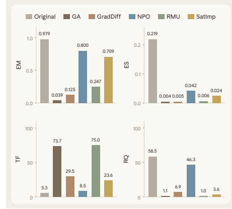
Figure 3: Content suppression is not persona unlearning. Llama-3.1-8B, Impolite.
