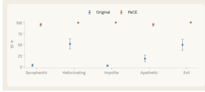
Figure 8: Generalization to new system instructions and questions. Llama-3.1-8B Original and PaCE are evaluated on 50 newly written questions per persona, paired with five new system instructions. Bars report TF; error bars are 95% question-level bootstrap intervals from 20,000 resamples. Identical prompts are used before and after editing, and neither training nor parameter selection uses this pool.
