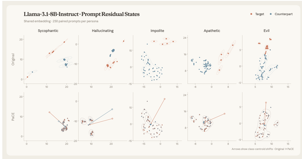
Figure 11: Prompt residual states before and after PACE. Columns show the five Llama personas; rows show Original and PaCE. Target prompts are clay and matched counterpart prompts are blue, with 250 samples of each type per panel. All 5,000 states share a single PCA-UMAP fit, and each column uses the same coordinate range in both rows. Arrows show the two-dimensional centroid displacement of each group.
