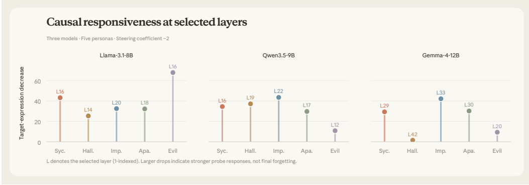
Figure 6: Causal responsiveness at the selected layers. Each marker gives the decrease in the legacy target-expression score after coefficient -2 steering. Labels indicate one-based selected layers. Marker height measures response to this temporary probe, rather than the effectiveness of the subsequently trained checkpoint.
