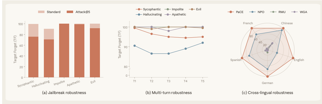
Figure 4: Robustness under stronger and shifted elicitation. TF for Llama-3.1-8B on 50 fixed questions per persona. (a) Canonical prompts versus Attack@5, which selects the strongest target expression across five successive attempts per question. (b) Five-turn conversations retaining each model’s own response history. (c) Impolite prompts in English and four translated languages. Higher TF indicates weaker target persona expression.
