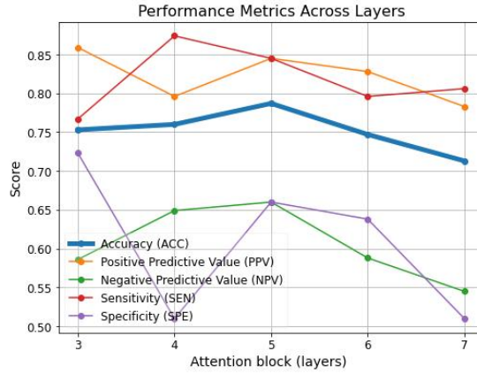
Fig. 5. The plot shows the variation in performance as the number of attention block (layers) increases.
