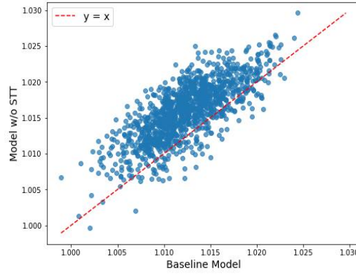
Fig. 4. Scatter plot comparing token cosine similarity distances between the TokenSTFormer and that without STT.
