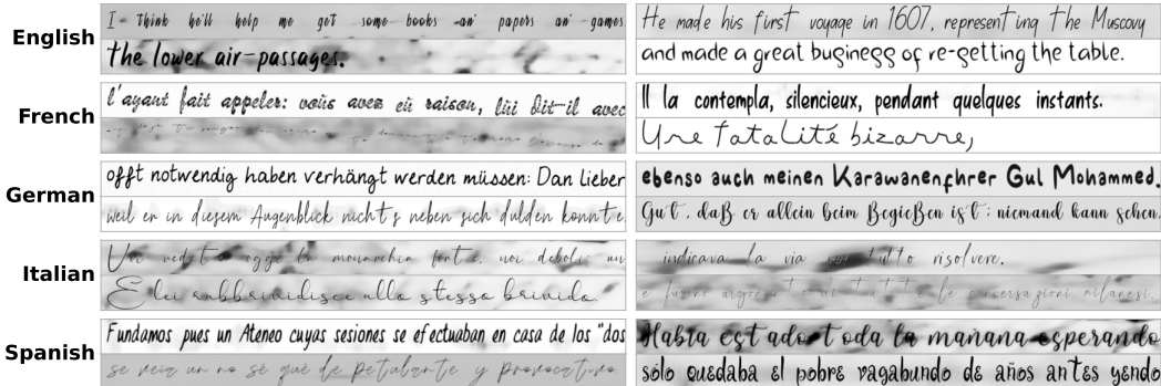
Figure 6: Synthetic handwriting samples used for SSL pretraining. Two examples per language (English, French, German, Italian, Spanish) drawn from our synthetic corpus, rendered from CulturaX and Gutenberg text with handwriting fonts and per-line variation in font, ink intensity, paper background, slant, baseline jitter, and inter-word spacing. Each sample is a 64 \times 1024 grayscale line image, the same resolution used by all SSL methods during pretraining.
