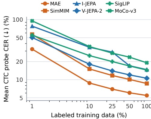
Figure 5: Label efficiency of frozen SSL encoders. Mean test CER (% , ↓) of probes with a BiLSTM readout and CTC loss trained on nested labeled subsets, averaged equally over all real HTR benchmarks. Orange denotes pixel reconstruction methods, blue JEPA methods, and green contrastive methods; markers distinguish methods within each family. Both axes are logarithmic.
