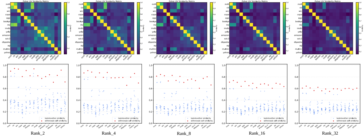
Figure 4: Ablation on the detection rank r_{\text{det}} for Fisher subspace similarity computation. A moderate rank provides a stable separation between within-task self-similarity and task-to-other similarity.
