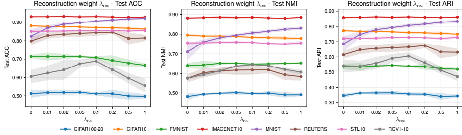
Figure 23: Sensitivity to the reconstruction weight \lambda_{\text{rec}} . Each panel reports test ACC, NMI, or ARI across datasets (mean \pm std over 5 runs).
