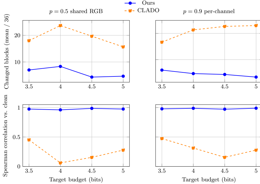
Figure 2: Allocation stability under corrupted calibration for our method and CLADO. Top: changed blocks (lower is better). Bottom: Spearman correlation with the configuration \mathbf{b} calculated with a clean dataset (higher is better). Values are averaged over three calibration seeds. Our method changes fewer block bit-widths than CLADO and better preserves their ordering under both calibration corruptions.
