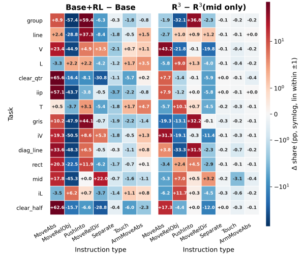
Figure 6: RL affects instruction distributions. RL from the base model broadly rewrites the instruction distribution, while RL after mid-training makes localized edits.
