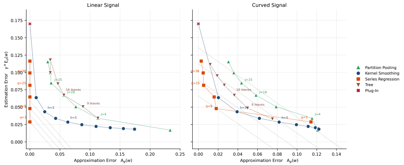
Figure 6: Every candidate is one point in terms of approximation error A_g(w) and estimation error \gamma^* E_\sigma(w) . Note that the axis are on different scales. Better smoothers lie closer to the bottom-left corner.
