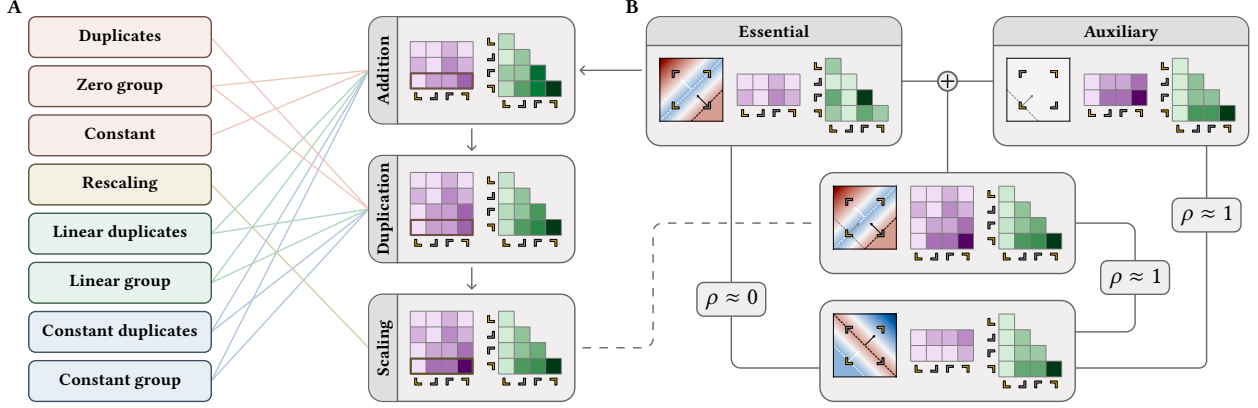
Figure 2: Primitive feature transformations unify parameter symmetries and separate essential from auxiliary geometry. (A) Parameter symmetries decompose into three primitive feature transformations and their inverses: addition , duplication , and scaling . Shown are their effects on hidden activations and RSMs when adding a zero-readout neuron to a solution in Panel B of Figure 1, duplicating it, and rescaling both copies. (B) Decomposing the full RSM of the resulting network (center) into essential and auxiliary contributions reveals the source of the dissociation in Figure 1. Whereas the essential component is nearly uncorrelated with the RSM of an opposite-family solution, the auxiliary component is nearly perfectly correlated with it, driving the full RSM toward the reference geometry without changing the function being computed.
