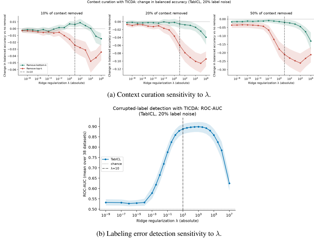
Figure 6: TICDA sensitivity to \lambda regularization.
