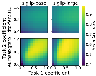
Figure 2: Performance landscapes across model scales. We visualize mean accuracy over a grid of merging coefficients. The heatmaps show highly similar distributions, indicating that the overall shape of the performance landscape is preserved across different model sizes.
