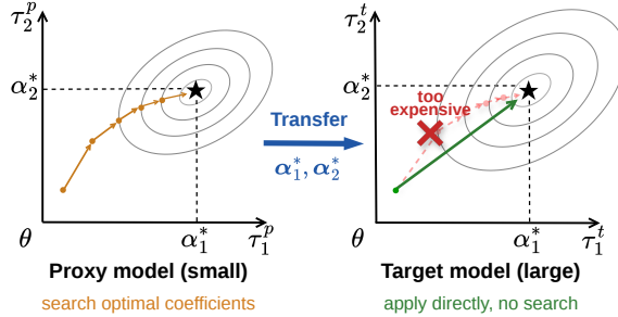
Figure 1: Overview of \alpha Transfer. Axes represent task vectors (\tau_1, \tau_2) ; superscripts p, t denote proxy and target models. Contours show the performance landscape when merging with coefficients (\alpha_1, \alpha_2) . Optimal coefficients found on a cheap proxy model transfer directly to the large target, skipping the expensive search.
