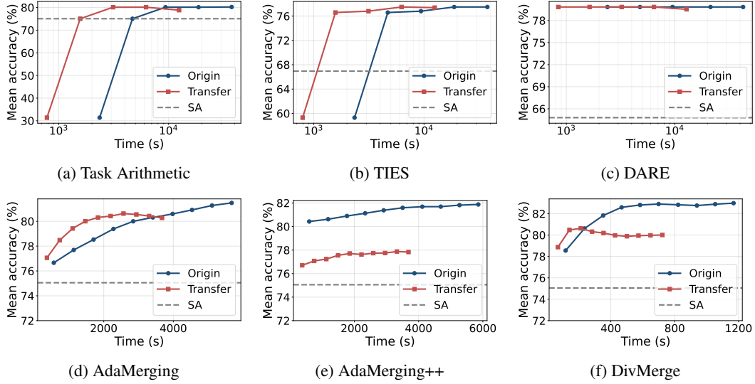
Figure 3: Budget analysis on SigLIP models. We compare the best achievable accuracy under varying computational time budgets for direct search (Origin) and \alpha Transfer (Transfer), with simple average (SA) as a static baseline. Transfer shifts the performance curves significantly to the left, reaching comparable accuracy in a fraction of the time for most methods. The performance gap in AdaMerging++ is further investigated in Appendix C.1, with full results provided in Appendix C.
