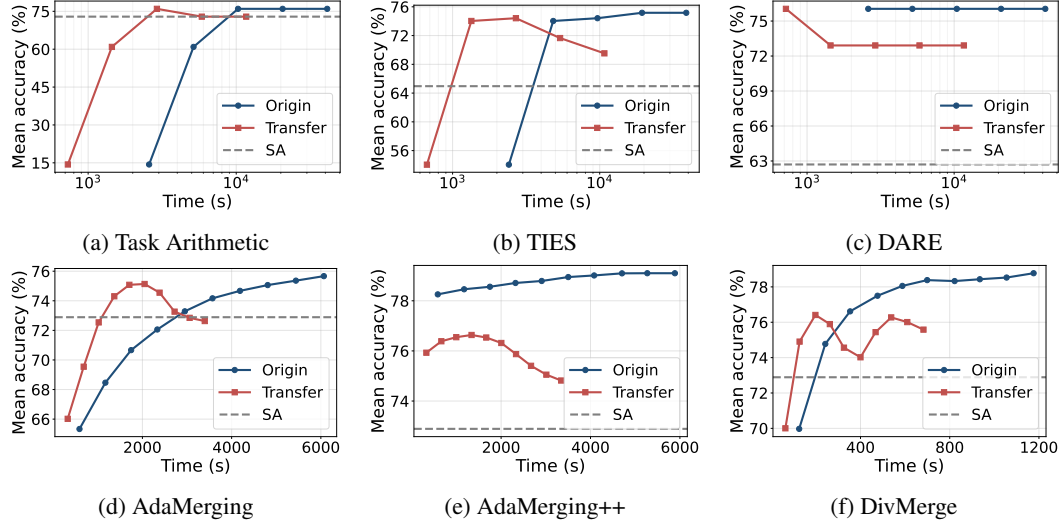
Figure 5: Budget analysis on ViT-B/16 \rightarrow ViT-L/14. We compare direct search (Origin) against coefficient transfer ( \alpha Transfer) under varying time budgets. Dashed lines indicate the simple average (SA) baseline. Top and bottom rows show evaluation- and gradient-based methods, respectively. Consistent with previous observations, \alpha Transfer shifts the performance curves to the left, reaching comparable accuracy in a fraction of the time.
