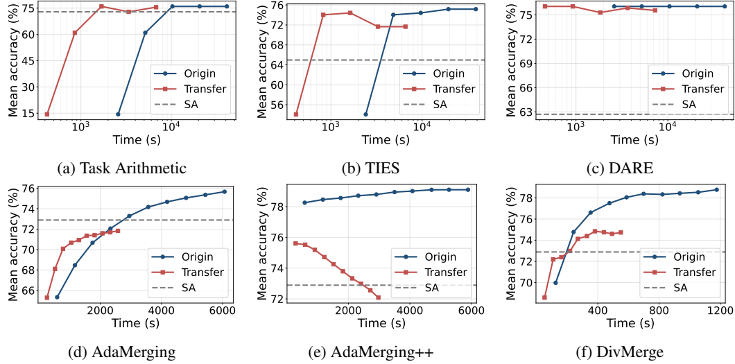
Figure 4: Budget analysis on ViT-B/32 \rightarrow ViT-L/14. We compare direct search (Origin) against coefficient transfer ( \alpha Transfer) under varying time budgets. Dashed lines indicate the simple average (SA) baseline. Top and bottom rows show evaluation- and gradient-based methods, respectively. Consistent with the SigLIP results, \alpha Transfer shifts the performance curves to the left, reaching comparable accuracy in a fraction of the time.
