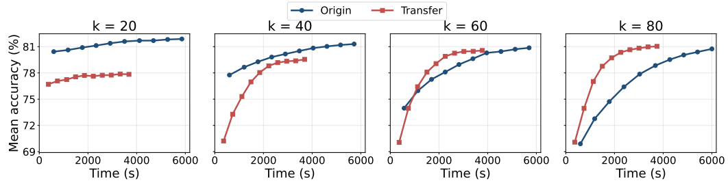
Figure 6: Impact of sparsity on \alpha Transfer in AdaMerging++. We compare exhaustive target optimization (Origin) against \alpha Transfer across varying TIES retention ratios k \in \{20, 40, 60, 80\} on the SigLIP-Base \rightarrow SigLIP-Large scaling chain. The x-axis represents the wall-clock training time. The effectiveness of \alpha Transfer is highly sensitive to the sparsity level: at extreme sparsity ( k = 20 ), direct target search achieves a higher performance ceiling. However, as the retention ratio increases ( k \geq 60 ), \alpha Transfer dominates the compute-performance trade-off, achieving massive speedups while converging to a higher final accuracy than direct target search.
