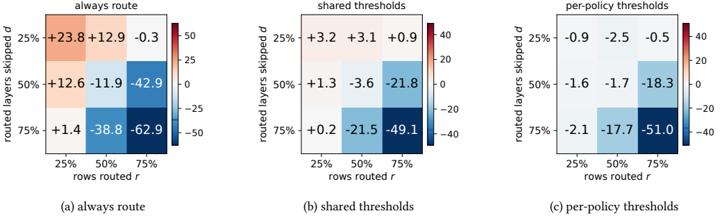
Fig. 3. Mean E2E change (%) against upstream for the nine RandomSkip arms at the GSM8K knee ( n=1 ), by rows routed r and routed layers skipped d , under the three switch settings (a–c).
