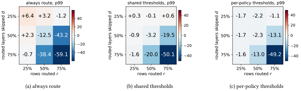
Fig. 6. p99 E2E change against upstream for the nine RandomSkip arms under the three switch settings, the same cells as Figure 3.
