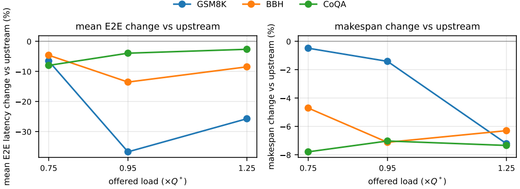
Fig. 5. Mean E2E change (left) and makespan change (right) against offered load, per workload, from the cells of Table 2.
