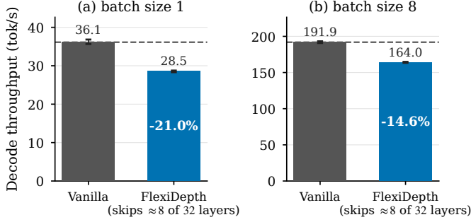
Fig. 1. Saved FLOPs are not saved time: decode throughput of the FlexiDepth checkpoint against its base model in a standard generation loop, with fixed batches of 1 and 8 requests each generating 256 tokens (mean of three runs; whiskers show the range).
