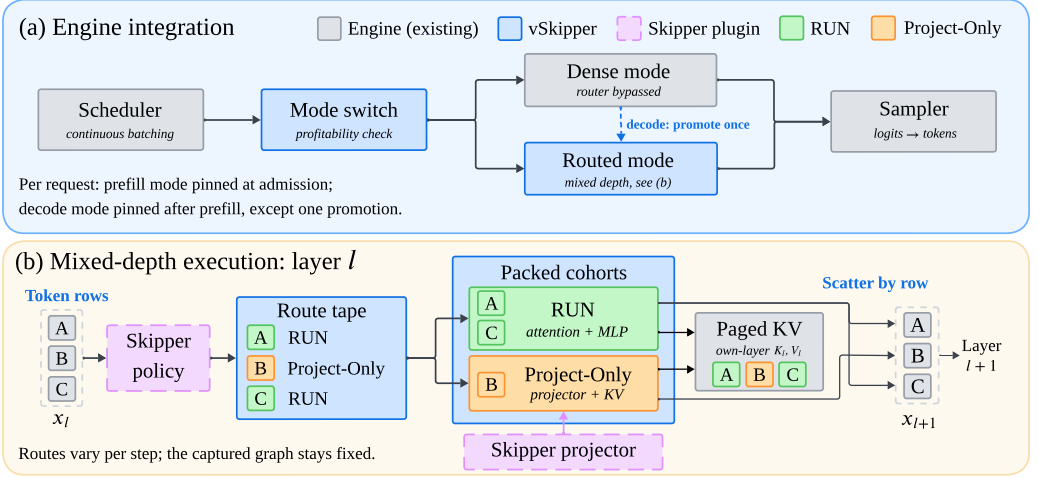
Fig. 2. Overview of vSKIPPER. (a) The mode switch selects dense or routed execution per request and phase based on predicted profitability (§3.3). (b) Routed layers record skipper decisions, pack rows into RUN and Project-Only cohorts, and scatter outputs back to the batch (§3.1). Project-Only rows still write their own-layer KV (§3.2).
