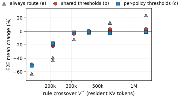
Fig. 4. The rule’s crossover V^* per RandomSkip arm against its measured mean E2E change under the three switch settings of Figure 3.
