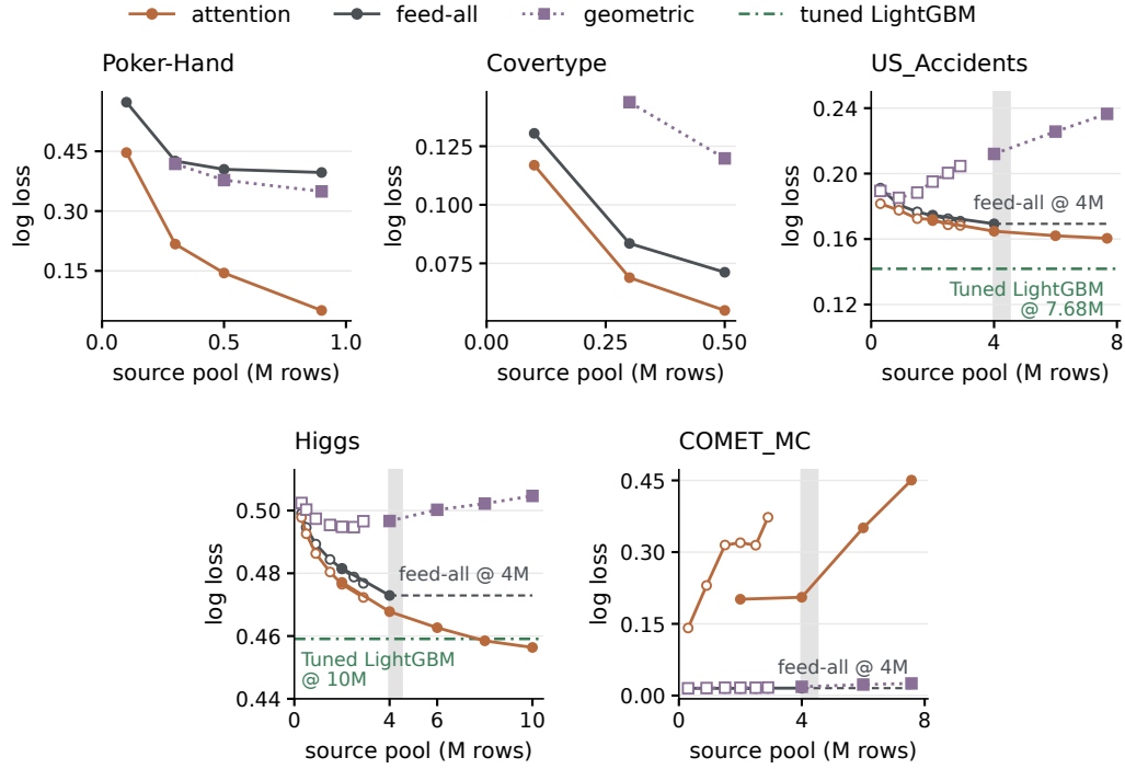
Figure 10: Complete source-pool sweeps with single-view TabPFN-3 on five large tables, including the geometric construction omitted from the main figure. Points are the five-seed mean log losses; each panel has an independent linear vertical axis. For the three largest tables, open and filled markers distinguish the 3M-subset and full-table splits; lines connect only points from the same split. Feed-all curves contain only measured values, ending at 4M where the pool exceeds capacity. Beyond 4M, dashed lines hold that reference fixed and gray bands mark the 4.0–4.5M capacity boundary. Green lines on US_Accidents and Higgs are tuned LightGBM endpoint references (Table 17).
