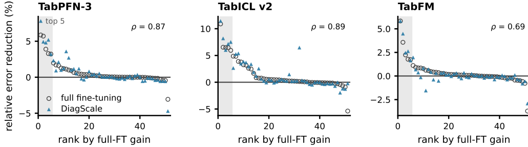
Figure 2: Per-dataset error reduction for DiagScale and full fine-tuning, relative to the same frozen backbone. Each panel orders 51 datasets by full fine-tuning’s reduction; shading marks its top five. \rho is the Spearman correlation between the two methods’ error reductions.
