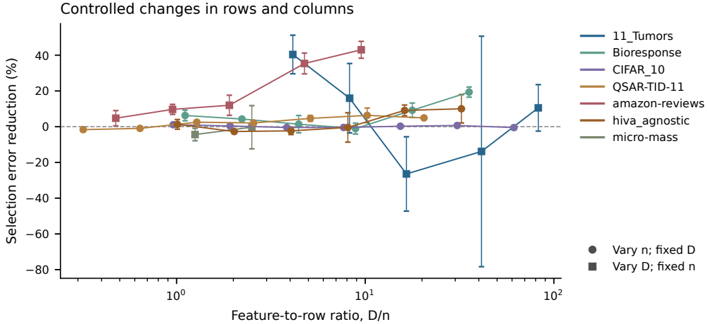
Figure 11: Column-curation controls at a fixed 200-column selection budget with single-view TabPFN-3, separate from the eight-view comparison in Table 22. Circles vary context rows at fixed width; squares vary width at fixed context size. The LightGBM ranking is fitted once per dataset and seed on the full training pool and held fixed through each sweep. Points are mean paired error reductions over four seeds, relative to using all available columns at that point; bars show one standard error. QSAR-TID-11 uses RMSE.
