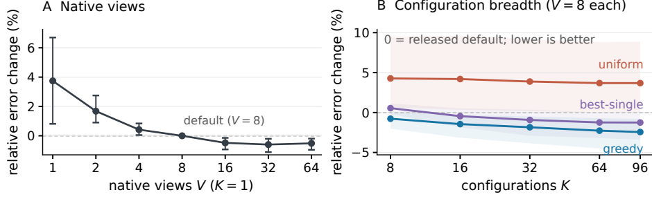
Figure 3: Aggregation on TabPFN-3. A : varying native views within one configuration. B : varying configuration count under three reducers, with eight native views per configuration. Errors are relative to the released eight-view default; negative values indicate improvement. Error bars and shaded bands show 95% confidence intervals. Complete curves appear in Figure 8.
