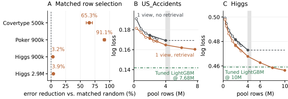
Figure 4: Row curation on frozen, single-view TabPFN-3. A : error reduction of attention-selected versus matched random rows; 95% paired t intervals over three seeds. B/C : five-seed mean log loss across source-pool sizes. Open and filled points use separate splits from 3M-row subsets and full tables, respectively. Curve labels in B also apply to C. Dashed lines show the no-retrieval loss at 4M rows; shading marks the 4.0–4.5M memory boundary on a single 80 GB GPU.
