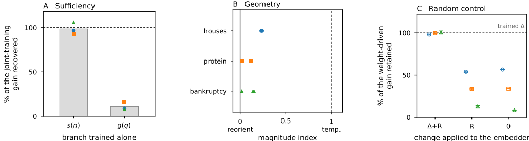
Figure 7: SoftScale component diagnostics. Blue circles, orange squares, and green triangles denote houses , protein , and bankruptcy . A: fraction of the joint-training gain recovered by separately training only the context-size branch s or the query-dependent gate g ; gray bars show the mean across datasets. B: each point summarizes one module group: the feature embedder or ICL stack, plus the classification decoder for bankruptcy. C: feature-embedder controls relative to its pretrained weights: trained change plus random perturbation ( \Delta + R ), random perturbation alone ( R ), or reversion ( 0 ); other scale modules remain trained. Error bars in C show standard deviations over five draws for \Delta + R and R . Gains in A and C are normalized by the corresponding loss reduction from jointly training both scale branches relative to pretrained weights along the same inference path.
