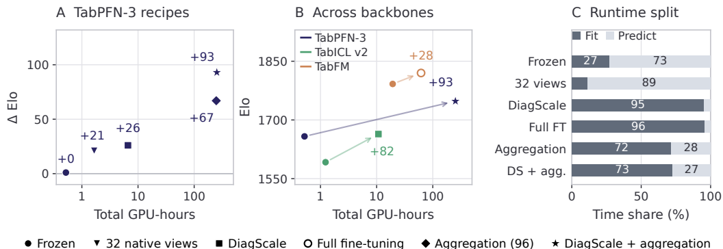
Figure 5: Performance and runtime on TabArena. (A) TabPFN-3 recipes. (B) Each backbone’s frozen model and highest-Elo evaluated recipe, connected by an arrow. Annotations show \Delta Elo relative to the corresponding reference baseline within each fit. (C) Fitting and prediction time shares for TabPFN-3 recipes. Runtime includes fitting and prediction across 51 datasets (Appendix E.4).
