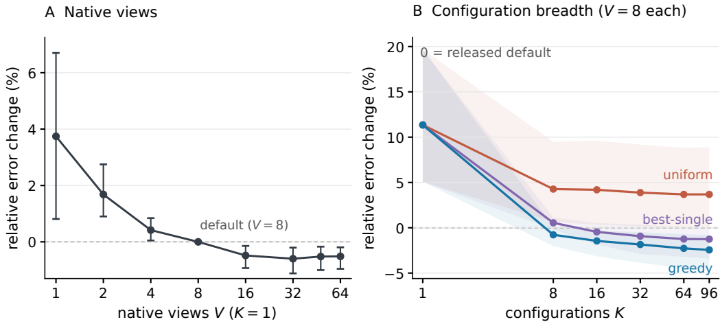
Figure 8: Complete aggregation curves, including native views below the released default and random single configurations. The three reducers coincide at K = 1 . Both panels use the same paired estimator and transformed 95% dataset-cluster bootstrap intervals as Figure 3, with independent vertical ranges and all intervals visible. The additional V = 48 point is included between the labeled 32- and 64-view ticks.
