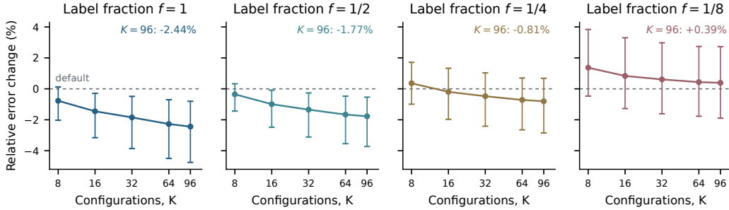
Figure 9: Greedy aggregation with different fractions of training-side selector labels. All panels share the same axes and fixed member predictions. Points use the dataset-weighted mean log-error ratio against the released default; bars show transformed 95% dataset-bootstrap intervals. Pool breadth improves each curve’s point estimates, while fewer selector labels reduce the gains. Intervals exclude zero for f \in \{1/2, 1\} and K \geq 16 ; all others include zero.
