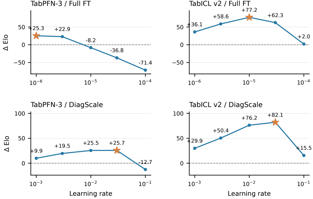
Figure 6: Learning-rate sensitivity for the cross-backbone adaptation comparison. Each point adds one candidate to the same 68 references; \Delta \text{Elo} is relative to the corresponding published default. Stars mark the rates with the highest unrounded \Delta \text{Elo} . All panels use five learning rates evaluated on the same 51 datasets.
