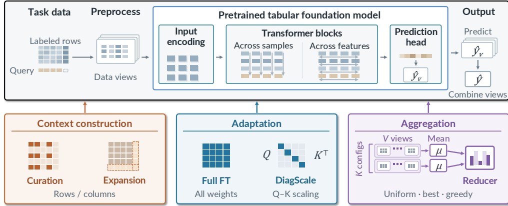
Figure 1: Three families of test-time compute modify different components of the inference pipeline. Top: an inference pipeline comprising preprocessing, a frozen tabular foundation model, and combination of predictions across data views. Bottom: context construction changes the conditioning data; adaptation changes model parameters; aggregation changes the prediction pool and the rule used to select or combine its members.
