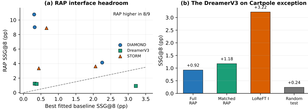
Figure 5: The dominant interface pattern and its exception. (a) RAP exceeds the strongest fitted editor in eight of nine cohorts spanning models and tasks. (b) DreamerV3 on Cartpole is the exception: Immediate LoReFT exceeds full RAP, RAP matched by norm, and its random test edit matched by norm. Delayed LoReFT is excluded from both panels.
