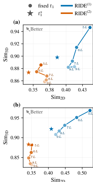
Figure 2: Comparison of Sim 2D vs. Sim 3D across t_1 \in \{nL\}_{n=5}^9 and t_1^* with L = T/10 . (a) conDitar-a; (b) IPDiff-a.
