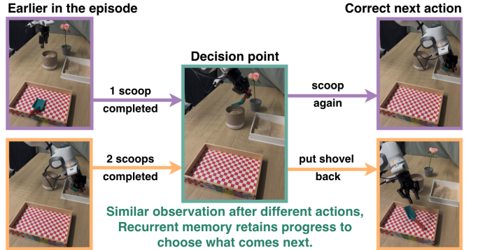
Fig. 1: Visually similar observations can require different actions depending on task history. ReCAT retains the completed scoop count in a compact recurrent memory, allowing the robot to scoop again after one scoop and put down the shovel after two.
