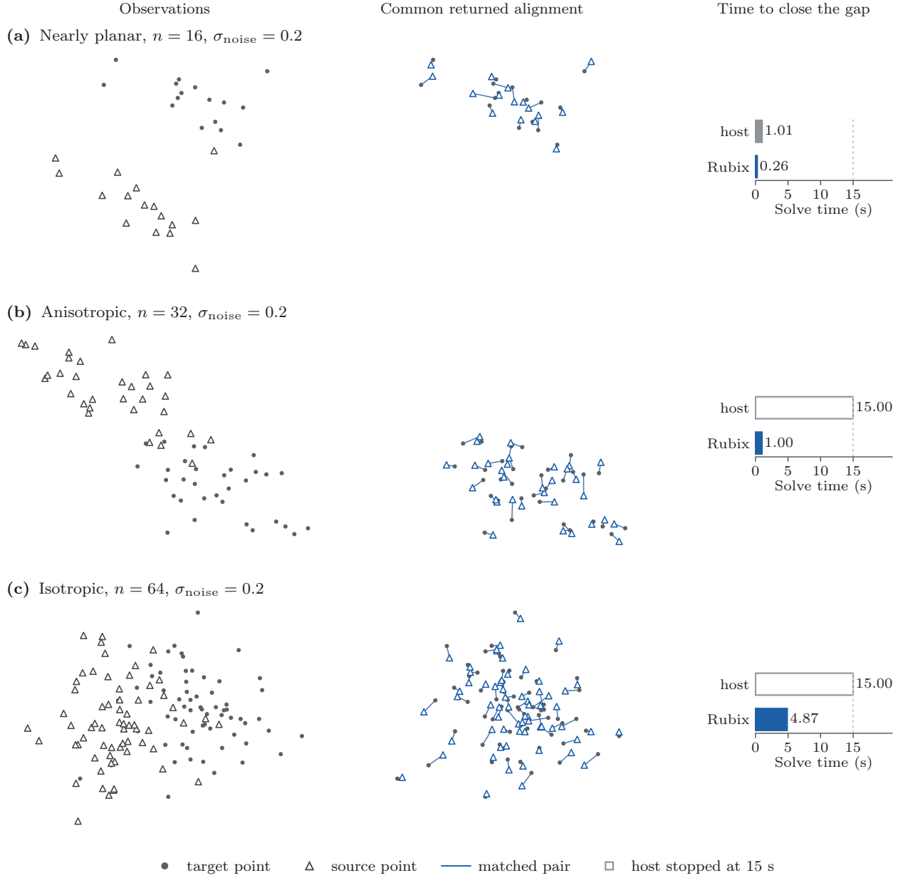
Figure A.6: Less search for the same SE(3) alignment. One favorable example per geometry, selected from all 72 scenes, including those on which the host reaches the time limit. The columns show the observations, the common fitted pose with its residuals, and the solve times; each row uses one viewpoint and scale. Hollow bars mark the limit of 15 s. At a target of 10^{-5} for the numerical gap in the mean squared error, Rubix closes all three cases, whereas the host with its rotation-cap bounds alone stops above the target in (b,c). Both variants return identical poses and matchings throughout the study.
