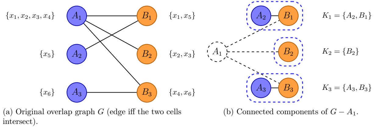
Figure 1: Illustration of Algorithm 1. In this example, the two deterministic predictors f_1 and f_2 induce signal partitions over the feature set. We write each signal cell by the feature indices it contains: \Pi_{f_1} = \{A_1, A_2, A_3\} , where A_1 = \{x_1, x_2, x_3, x_4\} , A_2 = \{x_5\} , and A_3 = \{x_6\} ; and \Pi_{f_2} = \{B_1, B_2, B_3\} , where B_1 = \{x_1, x_5\} , B_2 = \{x_2, x_3\} , and B_3 = \{x_4, x_6\} . Figure 1a shows the overlap graph G , whose vertices are the signal cells of f_1 and f_2 , and where an edge indicates a nonempty intersection between two signal cells. The cell A_1 is an articulation vertex. Figure 1b shows that G - A_1 has three connected components: K_1 = \{A_2, B_1\} , K_2 = \{B_2\} , and K_3 = \{A_3, B_3\} . By Algorithm 1, the cell A_1 is therefore split into the branch pieces A_1^{K_1} = A_1 \cap B_1 = \{x_1\} , A_1^{K_2} = A_1 \cap B_2 = \{x_2, x_3\} , and A_1^{K_3} = A_1 \cap B_3 = \{x_4\} . The remaining signal cells A_2 = \{x_5\} and A_3 = \{x_6\} are unchanged. Hence the finest constructible deterministic refinement of f_1 is \hat{\Pi}_1 = \{\{x_1\}, \{x_2, x_3\}, \{x_4\}, \{x_5\}, \{x_6\}\} .
