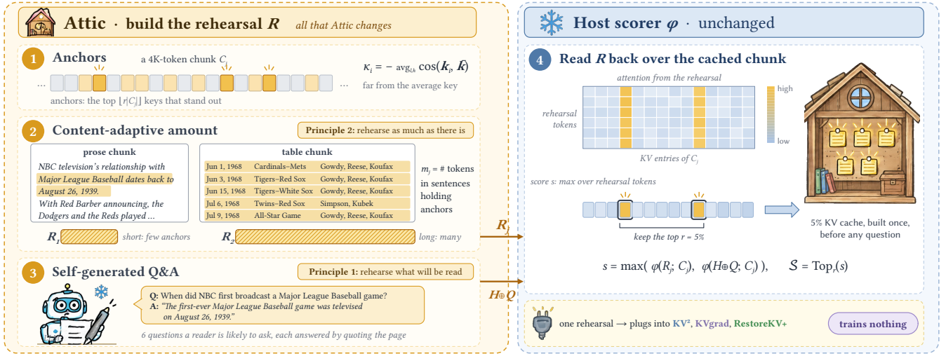
Figure 4: Overview of ATTIC. (Left) ATTIC builds the rehearsal R , the only part of compression it changes: ❶ the keys that stand out from the chunk’s average key are the anchors; ❷ the anchors are expanded to m_j tokens, the length of the sentences that hold them, so a prose chunk is rehearsed briefly and a table of facts at length (Principle 2); ❸ the model writes the questions a reader is likely to ask and answers them by quoting the page (Principle 1). (Right) The host’s scorer \phi reads the rehearsal back over the cached chunk, scores every KV entry by the attention it receives (heat map illustrative), and keeps the top r . Text is from the LooGLE page of Figure 1; the Q&A pair is the first one the model wrote for it. The same rehearsal plugs into KV^2 , KVgrad and RestoreKV+ , and nothing is trained.
