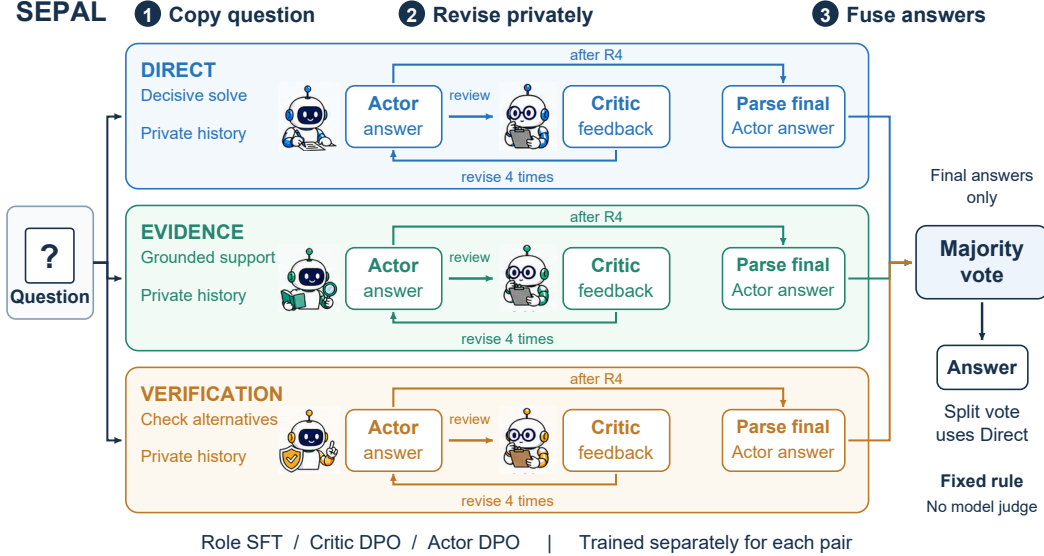
Figure 1: SEPAL in one view . A question enters three isolated role pairs, each refined through four private Critic-guided revisions (R1–R4). Only final parsed answers cross team boundaries. A fixed majority vote returns the prediction and uses Direct for split decisions.
