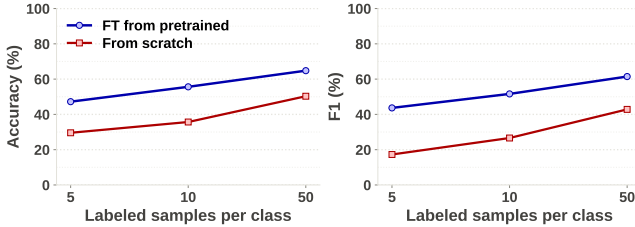
Figure 4: Few-shot downstream fine-tuning from pretrained versus random initialization, averaged over eight dataset-split pairs.
