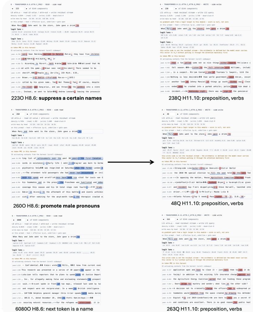
Figure 17: Connection between H8.6 (“S-inhibition head”) and H11.10 (“negative name mover head”). Components 2230 H8.6 (“suppress certain names”), 2600 H8.6 (“promote male pronouns”), 60800 H8.6 (“next token is a name”), which are the components that write the main functionality of H8.6 to the activation space, contribute strongly to the components 238Q , 48Q , 263Q H11.10 (“prepositions, verbs”).
