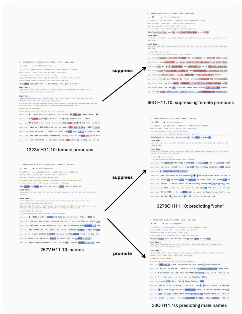
Figure 19: OV circuit of H11.10 (“negative name mover head”). The components 1323 V (“female pronouns”), 267 V (“names”) have a strong causal effect on 600 (“suppressing female pronouns”), 3278 O (“predict John”), 300 (“predict male names”). The components 600 O , 3278 O , 300 promote/suppress “male/female names/pronouns” and write the information to the activation space, which is the main role of H11.10 .
