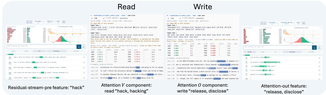
Figure 21: The image shows the component 5306 V (“hack, hacking”) at layer 5 reads the feature 16372 of residual-stream-pre which activates on “hack” context. 5306 V interacts with components 1454 O that fires on “release, disclose” and write out news related features 31334 at the output of the attention module.
