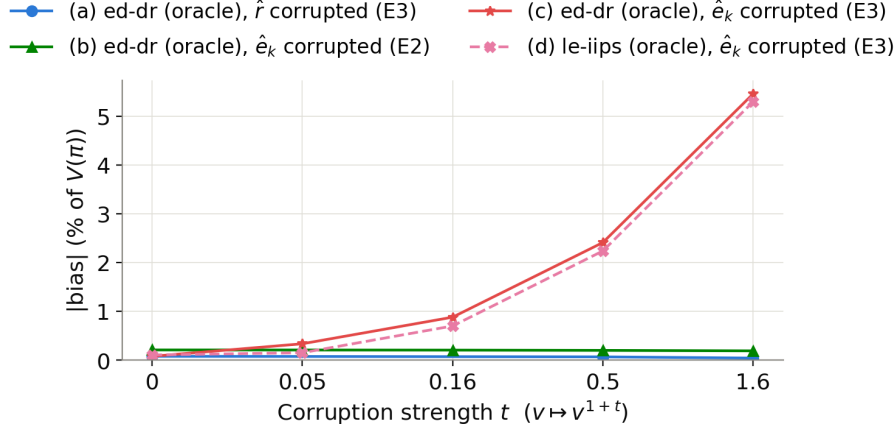
Fig. 3. |Bias| of ED-DR (oracle) against the size t of the error injected into one estimate. (a) \hat{r} corrupted under (E3); (b) \hat{e}_k corrupted under (E2); (c) \hat{e}_k corrupted under (E3), with (d) LE-IIPS (oracle) given the same \hat{e}_k for reference.
