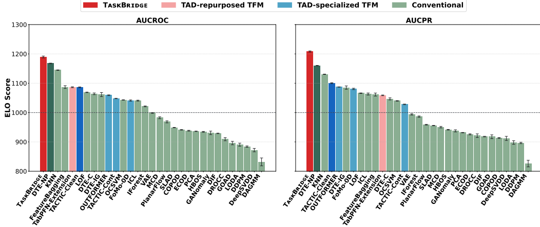
Figure 7: Elo score comparison across all baselines on all 790 ODDBench datasets. TASKBRIDGE achieves the highest Elo scores for both AUCROC and AUCPR, demonstrating consistently strong performance across diverse tabular datasets.
