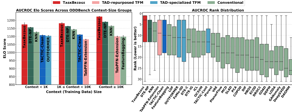
Figure 4: (Left) Elo scores across three ODDBench dataset groups with different context (training data) size (< 1K, 1K–10K, and ≥ 10K), showing the five methods with the highest average Elo scores in each group. (Right) Per-dataset AUCROC rank distributions across all baselines; colors follow Figure 1. TASKBRIDGE achieves the highest Elo score across all dataset groups and the strongest overall rank distribution. Corresponding AUCPR results are provided in Appendix C.1.
