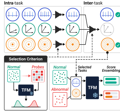
Figure 3: Overview of data-adaptive task selection. Candidates are evaluated with a pretrained TFM using nominal held-outs and structural-violation probes, and the most suitable tasks with proper configurations are retained.
