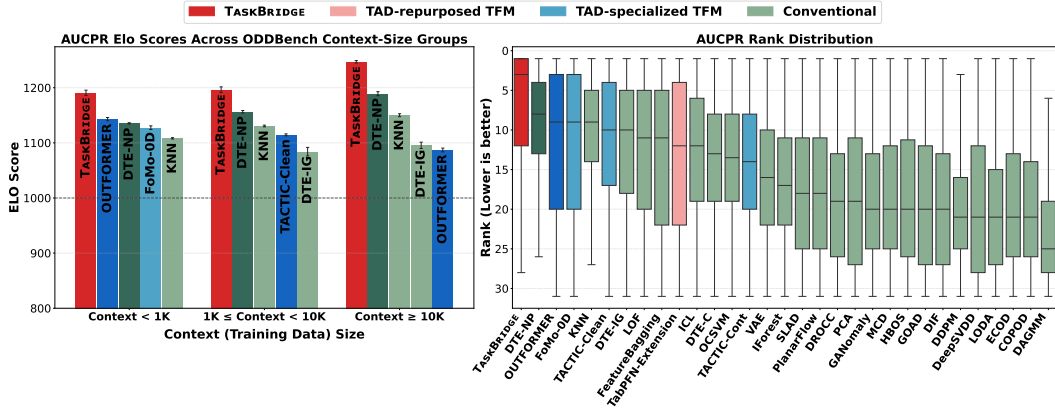
Figure 6: AUCPR performance comparison on ODDBench. (Extended results corresponding to Figure 4.) (Left) Elo scores across three dataset groups ( < 1K , 1K-10K , and \geq 10K ), showing the five methods with the highest average Elo scores in each group. (Right) Per-dataset rank distributions across all baselines; colors follow Figure 1. TASKBRIDGE also achieves the highest Elo score across all dataset groups with different context size and the strongest overall rank distribution for AUCPR.
