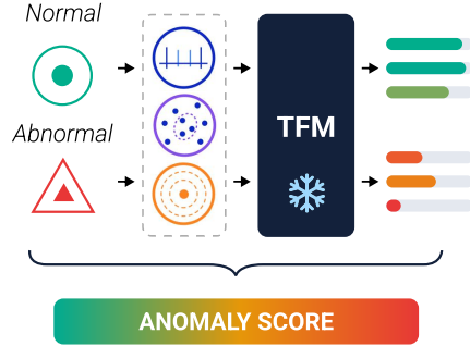
Figure 2: Overview of TASKBRIDGE. Given a query, it assigns its virtual targets under the designed supervised tasks and distinguishes normal and anomalous queries according to the predictive supports from the pretrained TFM.
