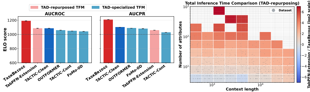
Figure 1: (Left) Elo scores of TFM-based TAD methods on ODDBench; darker colors indicate better performance. TASKBRIDGE achieves the highest Elo scores for both AUCROC and AUCPR. Full baseline comparisons are provided in Appendix C.1. (Right) Inference-time comparison between the TabPFN-Extension and TASKBRIDGE, with red indicating that TASKBRIDGE is faster. TASKBRIDGE scales more efficiently as both context length and dimensionality increase.
