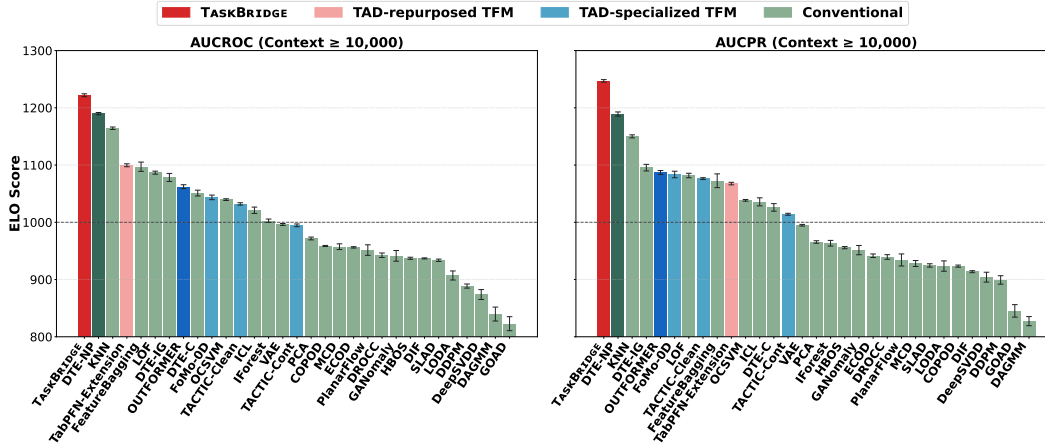
Figure 10: Elo score comparison across all baselines on partial ODDBench datasets with context (training data) size of at least 10K. TASKBRIDGE achieves the highest Elo scores for both AUCROC and AUCPR, maintaining strong performance with large amounts of normality-anchoring evidence.
