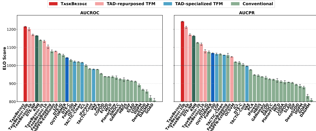
Figure 13: Elo score comparison across all baselines on 226 ODDBench datasets, including four TASKBRIDGE variants with restricted context budgets. Each TASKBRIDGE- i K variant limits the context size to i K samples. All variants, including the 1K setting, retain strong performance relative to the other baselines.
