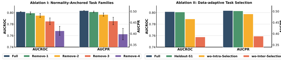
Figure 5: Ablation studies of TASKBRIDGE. (Left) Effect of the instantiated normality-anchored virtual tasks. Remove- i denotes removing i tasks from the five task templates introduced in Section 3.3; error bars indicate the variation across different removal combinations. The full task family achieves the best average performance. (Right) Effect of data-adaptive task selection. We compare the full procedure with a single held-out split, without intra-task selection, and without inter-task selection. The full selection procedure achieves the best overall performance.
