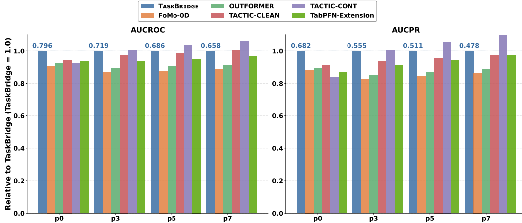
Figure 12: Robustness to context contamination on ODDBench. AUCROC and AUCPR performance are shown relative to TASKBRIDGE at each contamination level (TASKBRIDGE = 1), with its absolute performance reported above each group. p_k denotes the setting in which k\% of the context samples are replaced with anomalous samples. TASKBRIDGE remains competitive with TFM-based TAD baselines as contamination increases, while the contamination-specific TACTIC-CONT exhibits the strongest robustness under heavier contamination.
