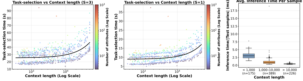
Figure 11: Inference-efficiency analysis of TASKBRIDGE. (Left, middle) Task-selection time across ODDBench datasets using 3 (default) and 1 held-out splits, respectively, as a function of context length and the number of attributes. (Right) Average inference time per test sample after task selection, grouped by context length; TASKBRIDGE maintains millisecond-level inference across all groups. Here, n denotes the number of datasets in each group: < 1,000 , 1,000\text{--}10,000 , and > 10,000 context length. Overall, TASKBRIDGE preserves efficient inference with TAD-repurposed TFM.
