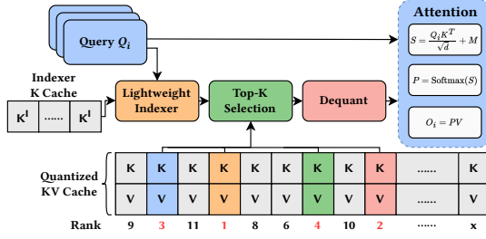
Figure 3. Illustration of the sparse attention workflow.
