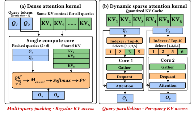
Figure 4. Comparison of the execution workflows of dense and sparse attention kernels.
