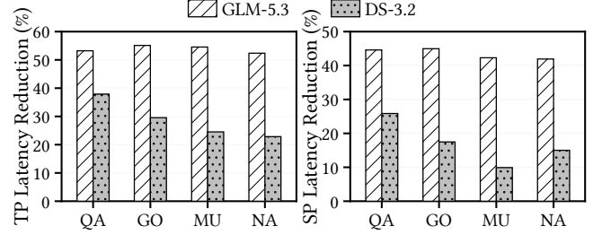
Figure 9. Average sparse-attention kernel latency reduction achieved by QUILT over OPS-Transformer on Qasper (QA), GovReport (GO), Musique (MU), and NarrativeQA (NA) from LongBench under SP and TP.
