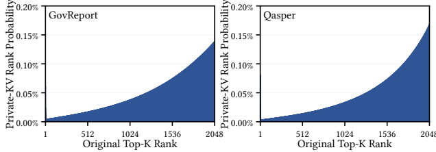
Figure 8. The ranking distributions of query-specific KVs.
