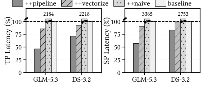
Figure 12. Average sparse-attention kernel latency under TP and SP, normalized to OPS-Transformer. Naive uses a Torch-based set-intersection implementation; Vectorized replaces it with SCSD; Pipeline further enables pipelined SCSD execution.
