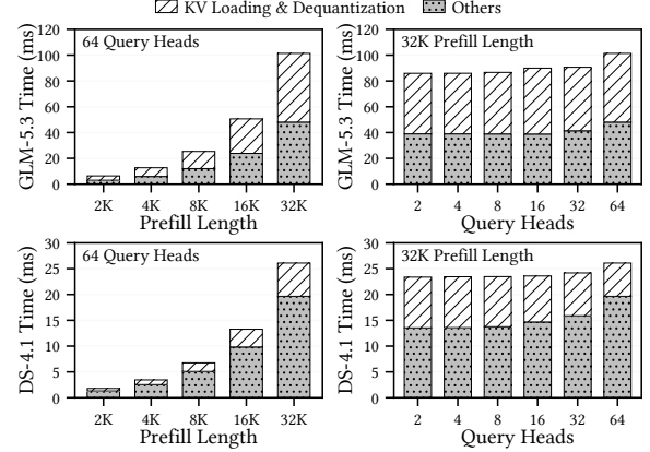
Figure 2. Latency breakdown of the existing sparse-attention kernel for GLM-5.3 and DeepSeek-4.1 on an Ascend 910C NPU across different prefill sequence lengths (SP) and query heads (TP).
