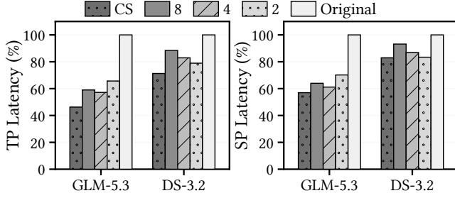
Figure 13. Average sparse-attention kernel latency of cascaded sharing (CS) and fixed query-group sizes of 2, 4, and 8 under TP and SP, normalized to OPS-Transformer.
