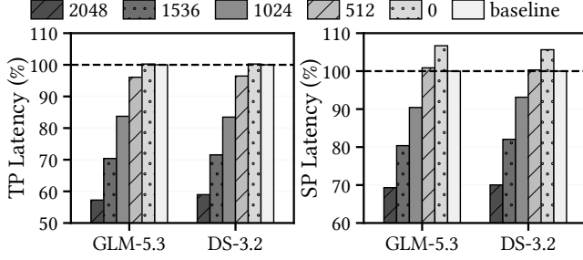
Figure 10. Average sparse-attention kernel latency with varying sharing lengths under SP and TP, normalized to OPS-Transformer.
