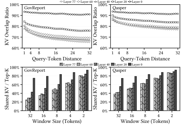
Figure 1. Top-K KV overlap ratios among neighboring queries across model layers and query-group sizes for GLM-5.3 [15] on the Qasper and GovReport datasets in LongBench.
