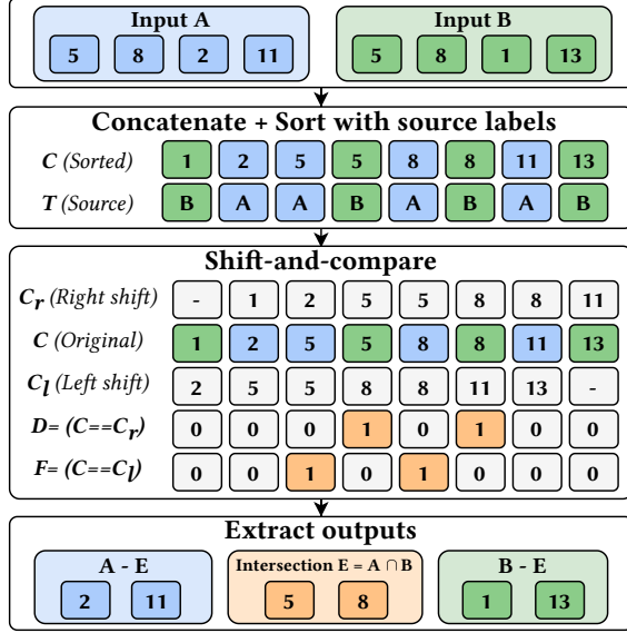
Figure 5. A running example of Shift-and-Compare Set Decomposition (SCSD) with two input KV index sets.
