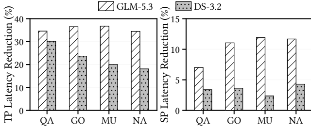
Figure 11. Average time-to-first-token latency (TTFT) reduction achieved by QUILT over OPS-Transformer on Qasper (QA), GovReport (GO), Musique (MU), and NarrativeQA (NA) from LongBench under SP and TP.
