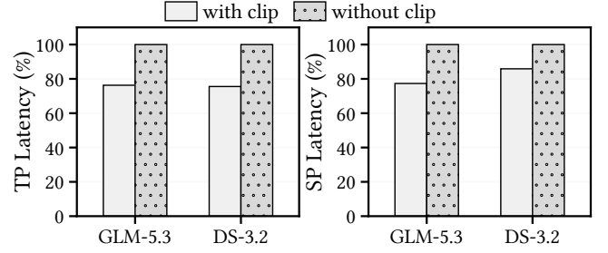
Figure 14. Average sparse-attention kernel latency with tile-aware clipping under TP and SP, normalized to the corresponding execution without clipping.
