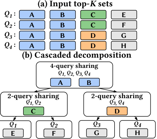
Figure 7. A running example of cascaded sharing across multiple query-group granularities.
