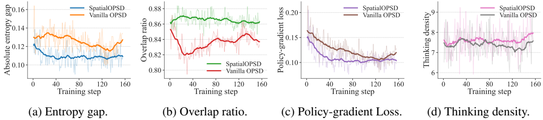
Figure 5: Training dynamics of SpatialOPSD-9B and vanilla OPSPD, both using Qwen3.5-9B as the backbone.
