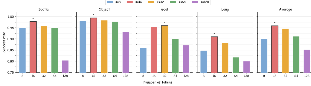
Figure 8: Effect of the number of action tokens on downstream VLA performance on the LIBERO benchmark. Performance improves from 8 to 16 tokens but degrades with larger token budgets, with 16 tokens achieving the best overall performance.
