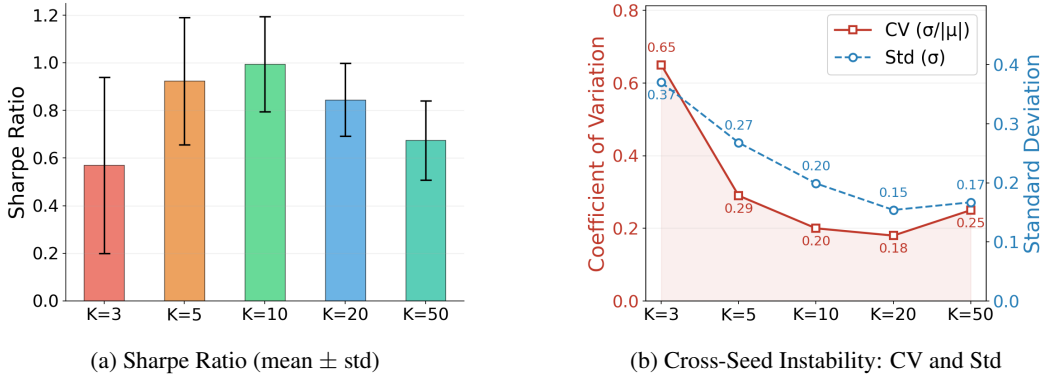
Figure 4: Effect of different top- K values on performance and stability across random seeds.
