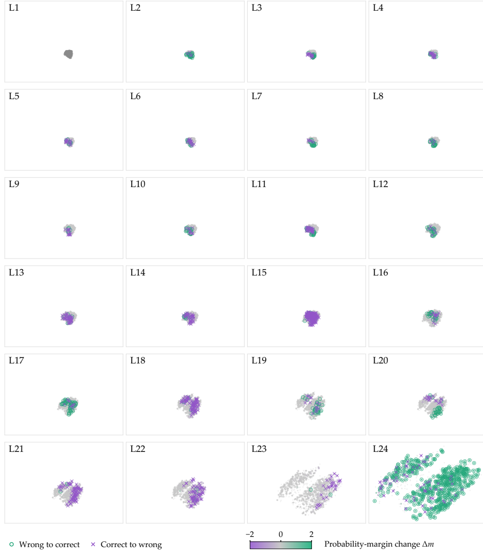
Figure 21: TabPFN-3 on Is-this-a-good-customer. All native layers in the fixed final-support PCA basis. Colors show adjacent probability-margin change under the frozen readout; rings and crosses mark corrections and deteriorations. The first layer is gray. Extraction and display conventions are given in Appendices A.1 and A.3.
