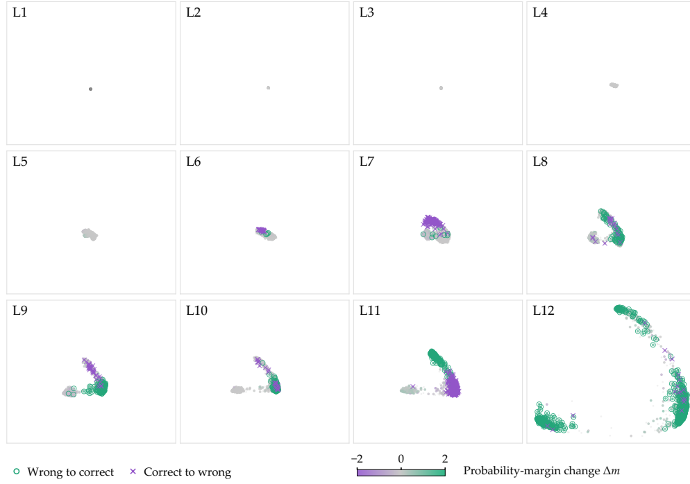
Figure 12: EXAONE-Tabular on SDSS17 . All native layers in the fixed final-support PCA basis. Colors show adjacent probability-margin change under the frozen readout; rings and crosses mark corrections and deteriorations. The first layer is gray. Extraction and display conventions are given in Appendices A.1 and A.3.
