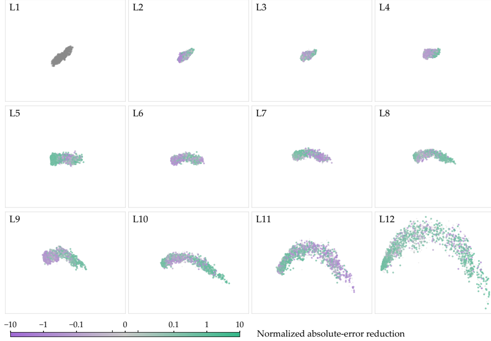
Figure 15: TabICLv2 on superconductivity. All native layers in the fixed final-support PCA basis. Green/purple indicate reductions/increases in absolute error under the frozen final-support Ridge readout, normalized by the support-target standard deviation. All four models share the same color scale. The first layer is gray; no binary correctness states are assigned.
