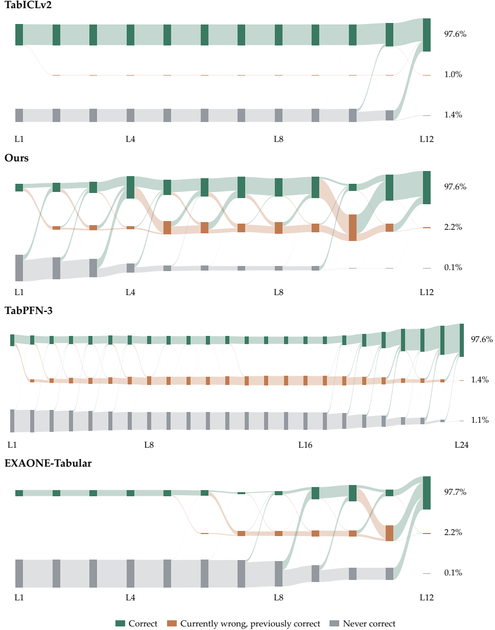
Figure 13: Four-model sample-state flows on SDSS17. Node heights and ribbon widths are percentages of all outer queries. Correct merges both currently-correct histories; the two wrong states distinguish whether a query was ever correct at an earlier layer. All native layers are retained.
