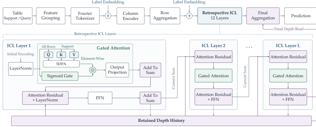
Figure 7: The RETRO architecture. A table encoder produces row representations for a retrospective ICL stack. Within each layer, separate aggregation modules construct attention and feed-forward inputs from available historical contributions. An input-conditioned gate modulates attention outputs before projection. Completed two-layer update groups remain available to subsequent layers and the final aggregation used for prediction.
