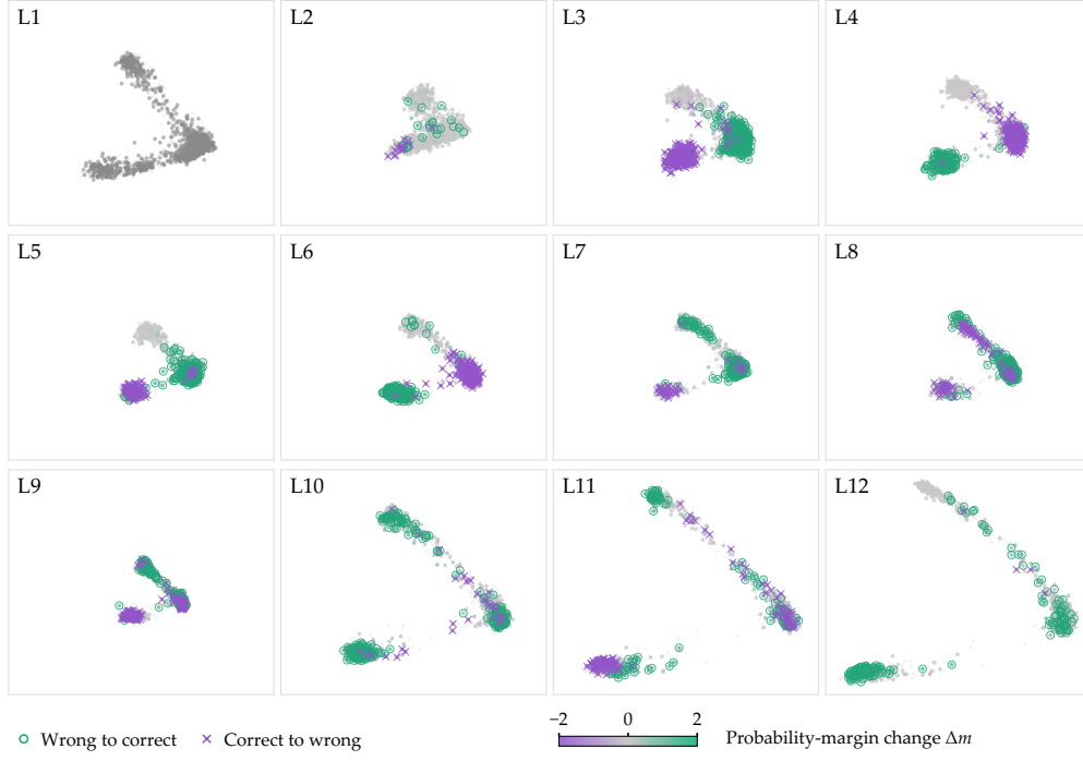
Figure 10: Our retrospective model on SDSS17. All native layers in the fixed final-support PCA basis. Colors show adjacent probability-margin change under the frozen readout; rings and crosses mark corrections and deteriorations. The first layer is gray. Extraction and display conventions are given in Appendices A.1 and A.3.
