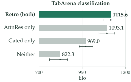
Figure 6: Component ablation. TabArena classification Elo within the four-configuration comparison. Whiskers: reported 95% intervals.
