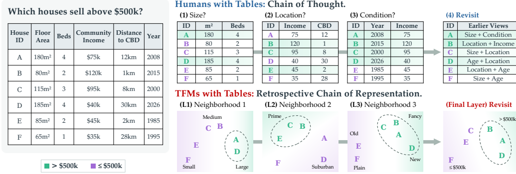
Figure 2: A housing example of complementary neighborhood views and retrospective integration. Top: a person considers size, location, and condition, then revisits these assessments to reach a decision. Bottom: the TFM schematic places the same homes in different neighborhoods across representations and integrates earlier information in the final representation. This illustrates a possible organization of tabular inference.
