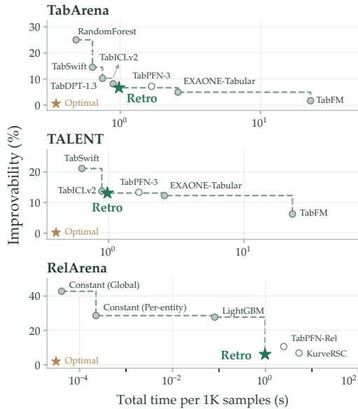
Figure 1: RETRO lies on the Pareto frontier of three mainstream benchmarks.
