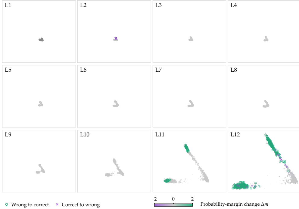
Figure 9: TabICLv2 on SDSS17 . All native layers in the fixed final-support PCA basis. Colors show adjacent probability-margin change under the frozen readout; rings and crosses mark corrections and deteriorations. The first layer is gray. Extraction and display conventions are given in Appendices A.1 and A.3.
