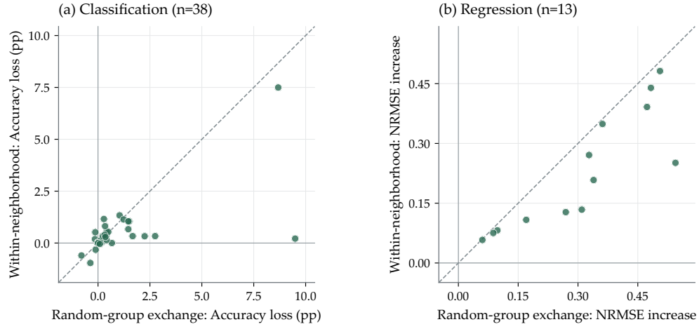
Figure 24: Neighborhood-constrained versus random gate exchange. Each point is a dataset, averaging three exchange seeds. Below the diagonal, exchange within support-derived neighborhoods is less harmful. Group sizes and moved-row counts are matched, within-neighborhood exchanges also induce smaller gate displacement.
