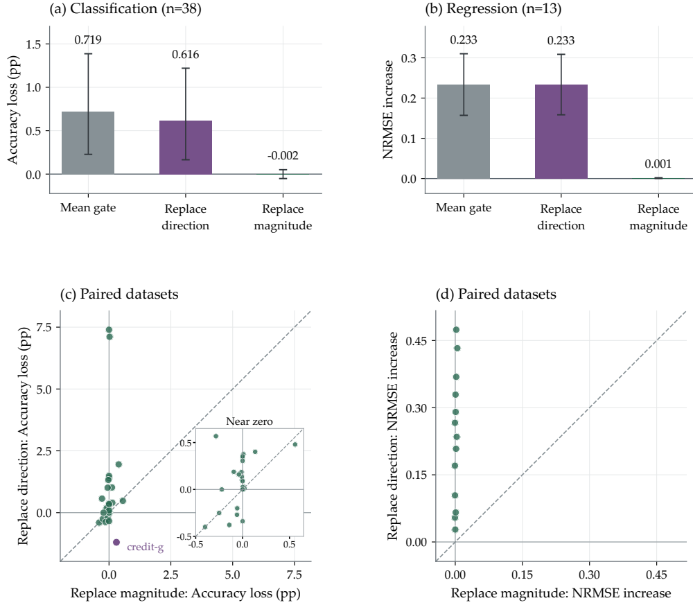
Figure 23: Sensitivity to update direction and magnitude. Top: mean degradation relative to learned gating, with 95% dataset-bootstrap intervals. Bottom: dataset-level effects; points above the diagonal indicate greater harm from replacing direction. The classification inset enlarges the region near zero. Positive values mean lower accuracy or higher NRMSE. Replacement distances are not matched.
