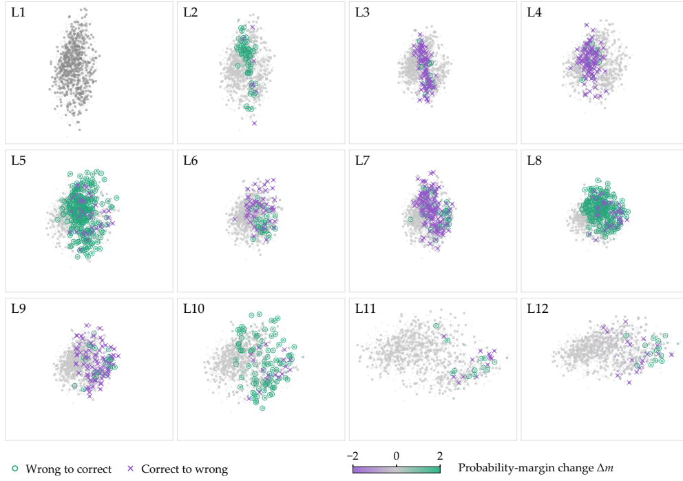
Figure 20: Our retrospective model on Is-this-a-good-customer. All native layers in the fixed final-support PCA basis. Colors show adjacent probability-margin change under the frozen readout; rings and crosses mark corrections and deteriorations. The first layer is gray. Extraction and display conventions are given in Appendices A.1 and A.3.
