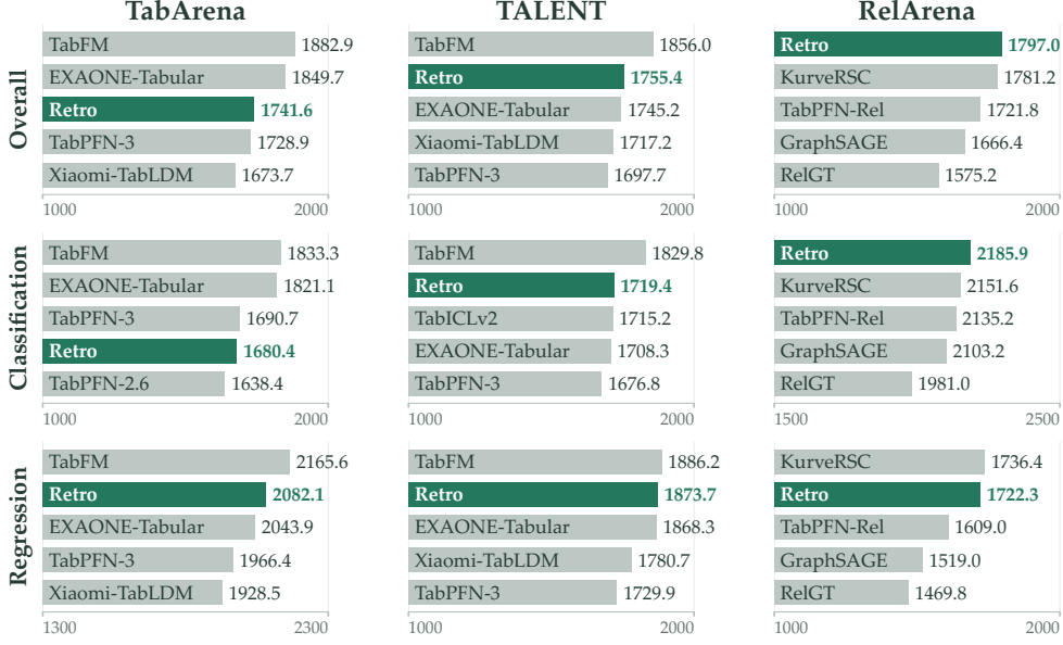
Figure 8: Elo rankings across three benchmarks. Each panel shows the five highest-rated methods. Candidate sets and scoring protocols differ, so ratings should be compared within panels. Complete rankings appear in Appendix E.
