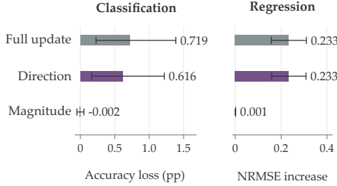
Figure 5: Gated-update geometry. Mean-gate replacement effects on 38 classification and 13 regression datasets in TabArena. Whiskers: 95% dataset-bootstrap intervals.
