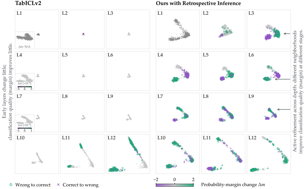
Figure 3: Layer-wise changes in predictive margin for TabICLv2 and a retrospective variant on SDSS17. The left and right grids show query representations across all 12 layers of TabICLv2 and our retrospective variant, respectively. Within each model, representations are projected onto a fixed PCA basis fitted to its final-layer support embeddings; coordinates are therefore comparable across layers within a model, but not between models. Color indicates the change in true-class probability margin from the preceding layer ( \Delta m ), with green denoting an increase and purple a decrease. Circles mark queries changing from incorrect to correct, and crosses mark the reverse. L1 is shown in gray because no preceding layer is measured. Insets enlarge L1, L4, and L7; the L4 and L7 insets use separately labeled, narrower color scales to reveal small early-layer changes. TabICLv2 exhibits limited directly readable changes through much of its depth, whereas the retrospective variant shows changes for different queries across more stages. Full four-model visualizations and aggregate results over 38 datasets appear in Appendices A.4 and C.1.
