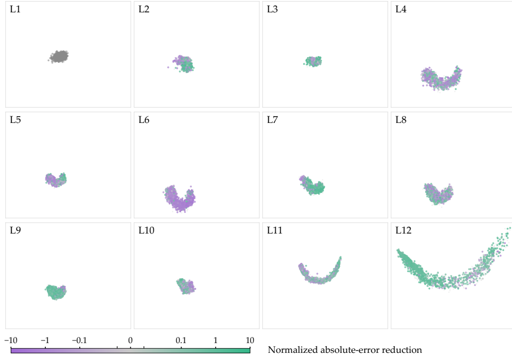
Figure 16: Our retrospective model on superconductivity. All native layers in the fixed final-support PCA basis. Green/purple indicate reductions/increases in absolute error under the frozen final-support Ridge readout, normalized by the support-target standard deviation. All four models share the same color scale. The first layer is gray; no binary correctness states are assigned.
