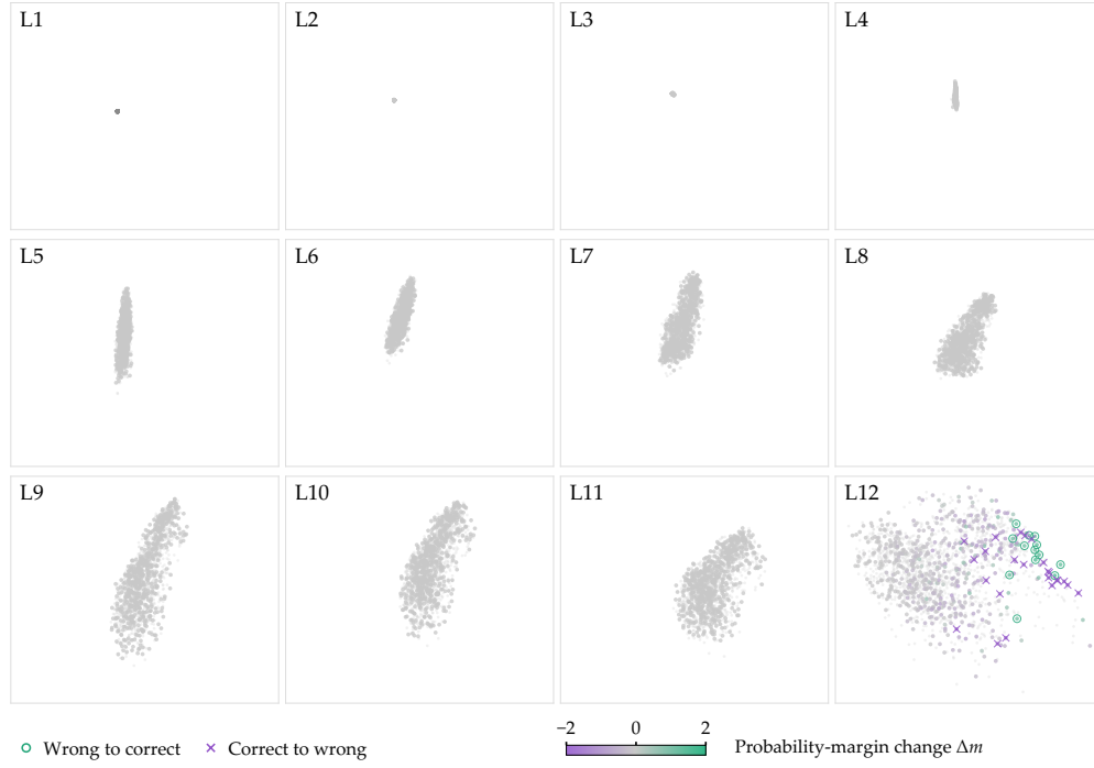
Figure 22: EXAONE-Tabular on Is-this-a-good-customer. All native layers in the fixed final-support PCA basis. Colors show adjacent probability-margin change under the frozen readout; rings and crosses mark corrections and deteriorations. The first layer is gray. Extraction and display conventions are given in Appendices A.1 and A.3.
