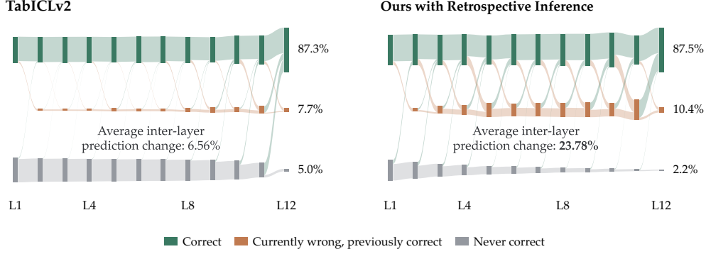
Figure 4: Sample-state flows across depth. Frozen-readout trajectories for TabICLv2 (left) and our ungated retrospective variant (right), averaged equally over 38 classification datasets. Correct merges always-correct and previously-wrong but currently-correct queries; the two wrong states distinguish whether a query was ever correct. Ribbon widths show query fractions across all 12 layers. The displayed average measures correctness switches over L1→L2 through L10→L11; only this summary excludes the final transition.
