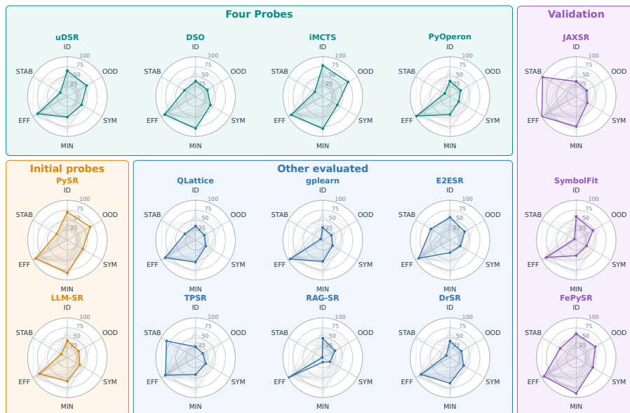
Figure 4: Per algorithm six axis profiles on Core50 . Each panel displays the six axis scores of one algorithm. Normalized scores are multiplied by 100 for a common 0 to 100 display scale. Gray profiles show the remaining algorithms for reference. The panels reveal differences beyond a single numerical ranking.
