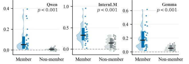
Figure 2: Teacher-directed audit projection for member and non-member prompts.
