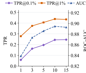
Figure 7: Sensitivity to R on Qwen-MATH under Full-distribution access.
