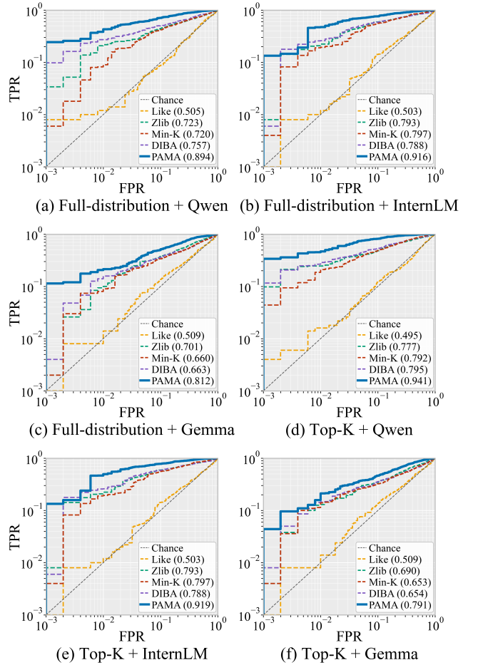
Figure 3: ROC curves on the MATH dataset under full-distribution and Top- K access, with ROC-AUC scores reported in parentheses in the legend.
