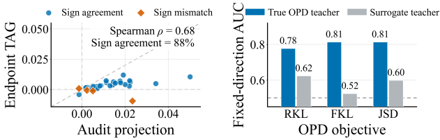
Figure 4: Validation of TAG. Left: agreement with the gradient-based audit projection. Right: fixed-direction AUC across OPD objectives and teacher references.
