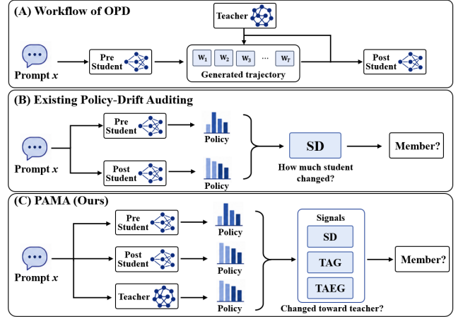
Figure 1: Overview of OPD prompt and membership auditing: (A) teacher-guided student training, (B) policy-drift auditing, and (C) PAMA with teacher-directed alignment.
