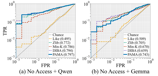
Figure 8: ROC curves under surrogate-teacher access without true OPD teacher model.
