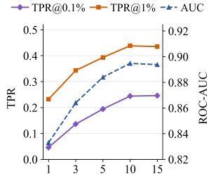
Figure 6: Sensitivity to K on Qwen-MATH under Top- K access.
