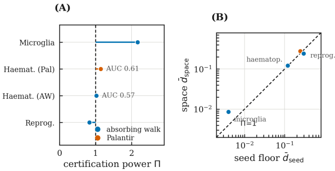
Fig. 4. Certification power. (A) \Pi for each of the four dataset–algorithm arms, with the area under the curve for -FM predicting clonally observed misassignment annotated on the two arms that carry lineage labels. Only the microglial arm exceeds \Pi = 1 appreciably. (B) The two components of \Pi per arm, model-space disagreement against the within-algorithm seed floor, on a logarithmic axis; an arm on the diagonal has \Pi = 1 and certifies nothing beyond seed stability.
