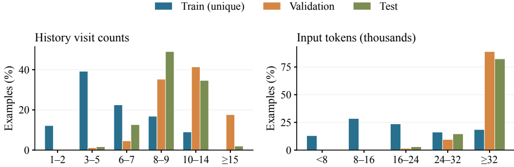
Figure 6: The distribution of historical visit counts and input tokens for each dataset.
