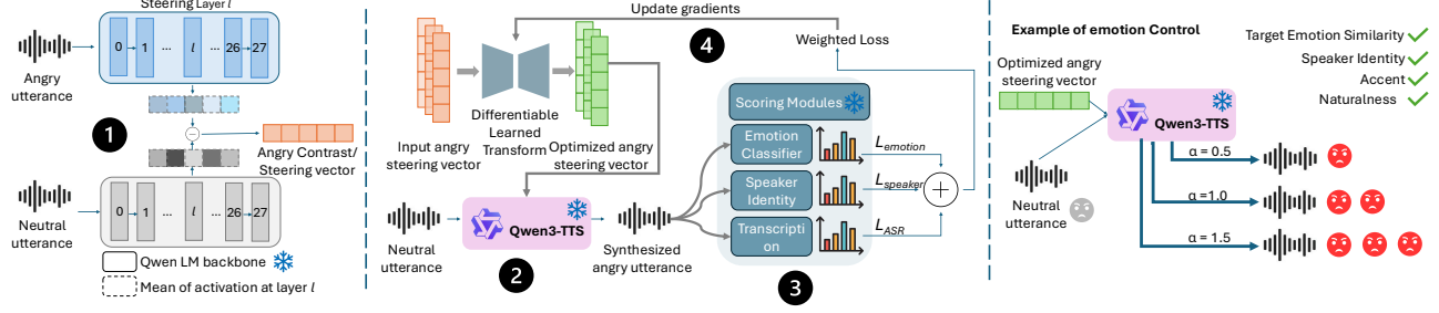
Fig. 1. SteerSpeech overview.
