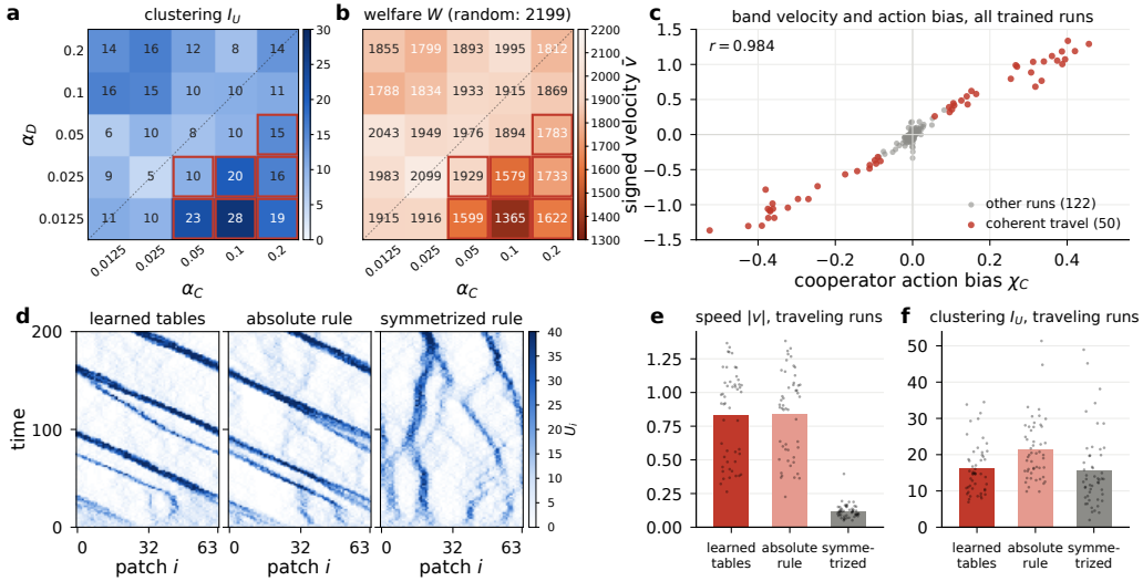
Figure 10: Complete learning-rate and directional-bias analysis of the 172 trained runs. (a,b) Cell means of clustering and welfare on the 5 \times 5 grid. Red boxes mark cells in which at least half of the seeds travel coherently, and the dashed line marks equal rates. (c) Signed velocity \bar{v} against the cooperators' action bias \chi_C for every trained run. (d) A fresh rollout of a ratio-4 run under the learned tables, the absolute rule, and the symmetrized rule. Figure 9 shows the same rollout enlarged. (e,f) Speed and clustering of the 50 coherently traveling runs under the three policies in the broad scan. Bars are means and dots are runs.
