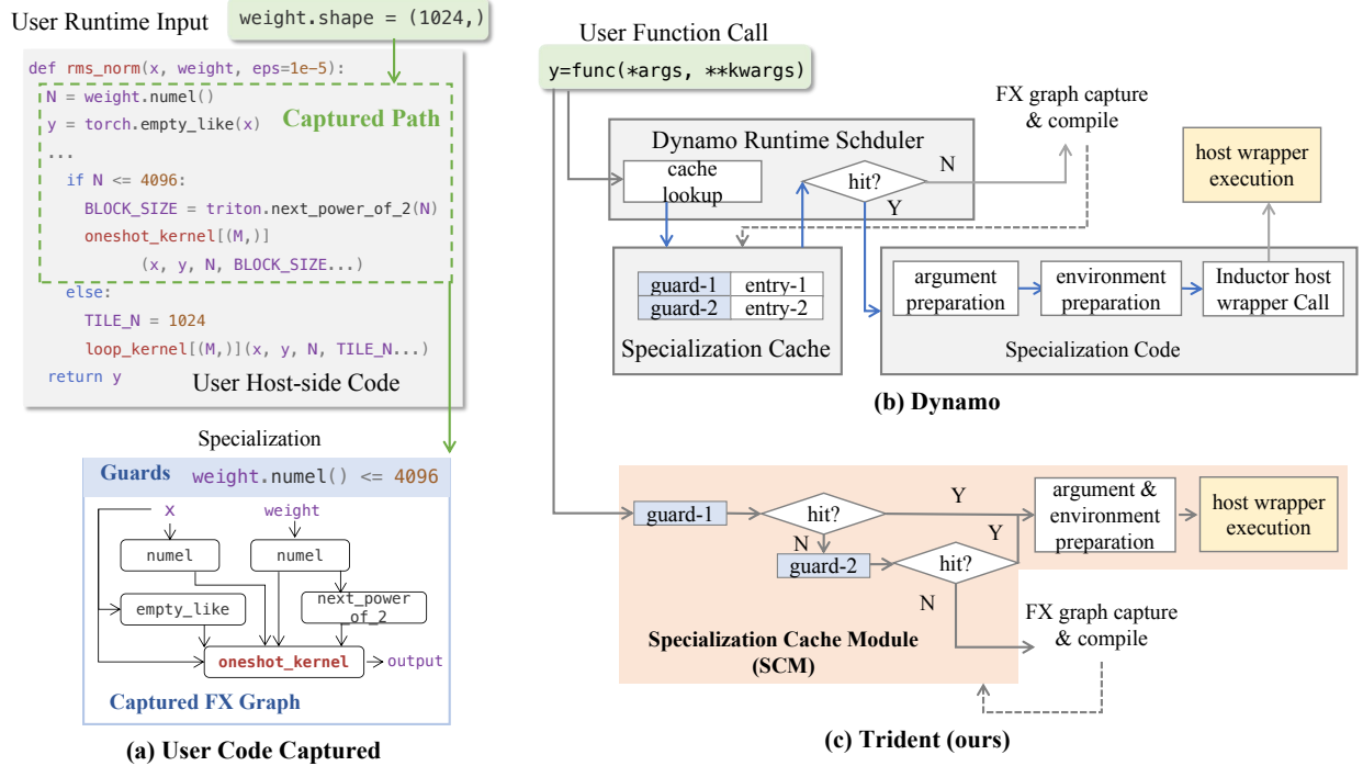
Figure 1. (a) An rms_norm example (omitted for clarity) with two Triton JIT kernels, onshot_kernel and loop_kernel . Different input shapes take different host-side paths; Dynamo captures the executed path as a guarded FX-graph specialization. (b) Dynamo runtime-managed execution model, where blue edges mark cross-layer and glue overhead between warm-path steps. (c) TRIDENT SCM-based execution model.
