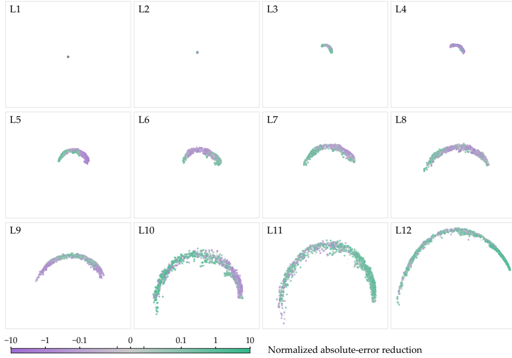
Figure 18: EXAONE-Tabular on superconductivity . All native layers in the fixed final-support PCA basis. Green/purple indicate reductions/increases in absolute error under the frozen final-support Ridge readout, normalized by the support-target standard deviation. All four models share the same color scale. The first layer is gray; no binary correctness states are assigned.
