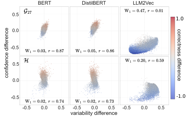
Figure 10: Differences on the training dynamics across encoders with synthetic (top) and human (bottom) data on dependency parsing. Same notation as in Figure 5.
