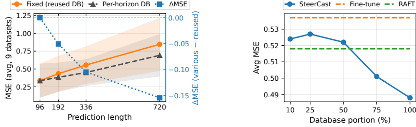
Figure 3: Database design ablations. (Left) Database protocol on Time-MoE, comparing a single reused database with per-horizon databases. (Right) ETTh2 with Time-MoE: forecasting MSE versus retrieval database size (10%–100%), with Fine-tune and RAFT as horizontal baselines.
