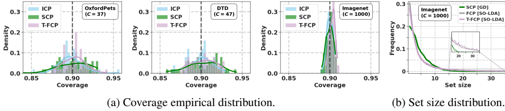
Figure 1: Analysis on empirical coverage and set size distribution on representative datasets. Results using CLIP ViT-B/16 as backbone, N = C \times 16 samples for calibration.
