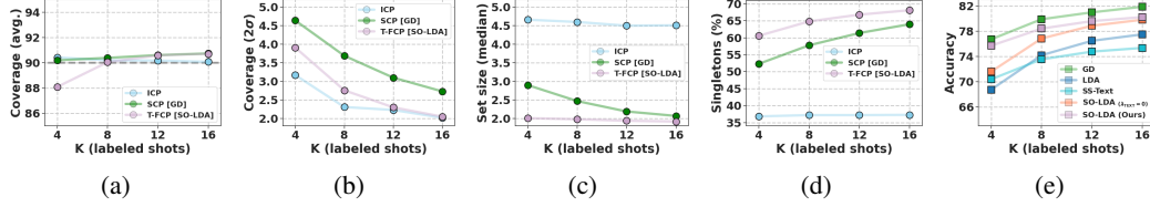
Figure 4: Studies at lower data regimes: (a-d) conformal procedures, and (e) few-shot solvers. Results using CLIP ViT-B/16 as backbone, and conformal sets at \alpha = 0.1 , averaged for 11 datasets.
