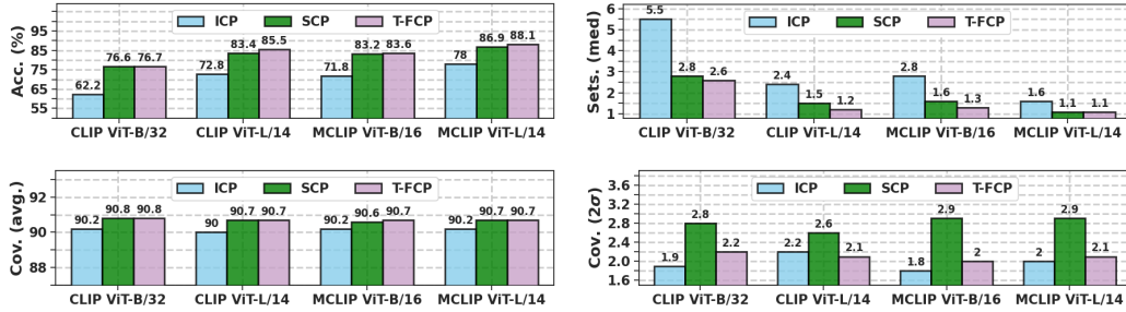
Figure 5: Generalization atop other CLIP [39] and MetaCLIP [58] backbones of conformal procedures. Results using N = C \times 16 samples and \alpha = 0.1 , averaged across 11 datasets.
