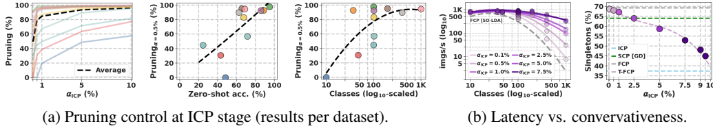
Figure 3: Ablation studies on T-FCP. Results using CLIP ViT-B/16 as backbone, N = C \times 16 samples for calibration, and conformal sets created at \alpha = 0.1 error rate.
