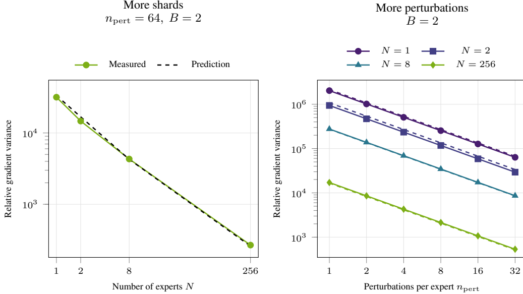
Figure 10: More shards and more perturbations reduce relative gradient variance. Lower is better. Centered estimator variance is divided by the squared exact gradient norm. Model size is roughly 8.44M in total (Section 3). Left, N = 256 has 118\times lower variance than N = 1 . Right, doubling n_{\text{pert}} halves variance and doubles update compute. Points use weights at 10,000 updates and the same two ensemble validation chunks on an RTX 5090. Dashed lines are predictions for the recorded perturbation distribution, without fitting. These tests measure variance at fixed weights, not learning speed. Appendix G.1 gives the calculation.
