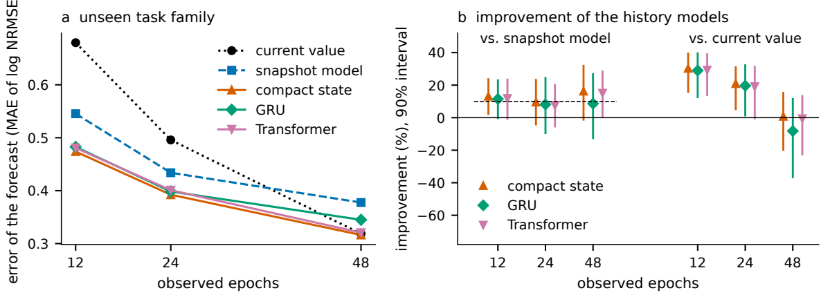
Figure 4: Forecasting screen with 1,000 runs for training the forecasters. a: forecast error with one task family held out. b: improvement of the three history models over the snapshot model (left) and over the current validation error (right), with 90% bootstrap intervals over families. The dashed line is the threshold set for epoch 48 against the snapshot model.
