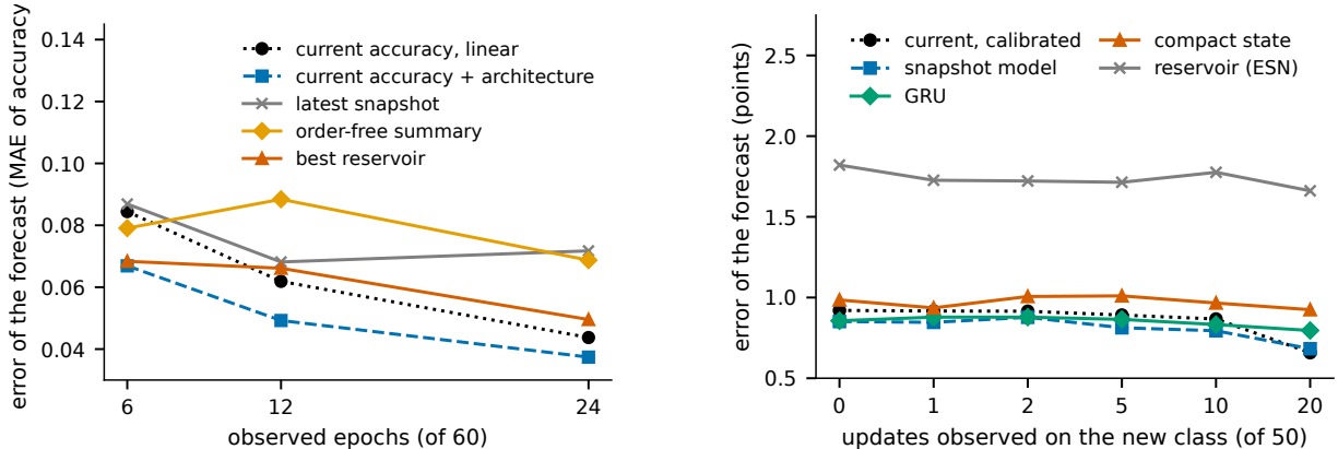
Figure 6: Left: CIFAR-100 screen, forecast error with a block of tasks held out; the unfitted current accuracy (error 0.287 to 0.136) is off the scale. Right: class-incremental screen, mean forecast error over five targets in percentage points with a class order held out.
