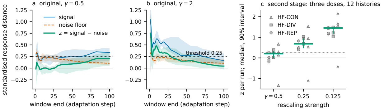
Figure 2: Positive control in the main study. a, b: original design on six histories. Lines are medians of the response distance to the unchanged checkpoint (signal), of the distance between two unchanged measurements (noise floor) and of their difference z , for averaging windows ending at each step; bands are 90% bootstrap intervals. c: second stage with stronger doses on 12 histories, window ending at step 85. Points are histories, bars are medians with 90% intervals. The dotted line is the threshold fixed before the first run.
