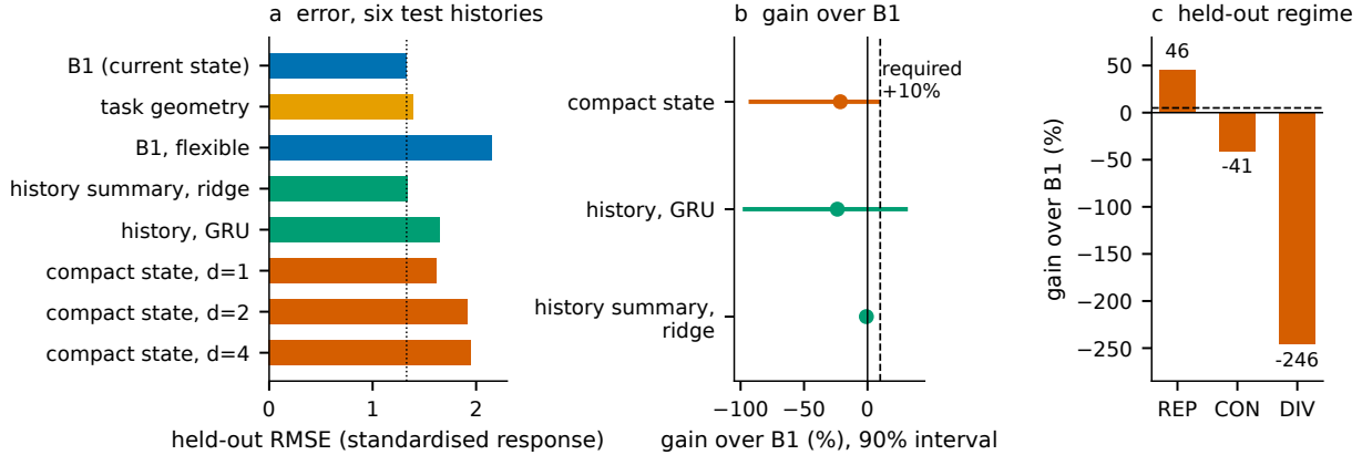
Figure 3: Prediction of the response to further training in the main study. a: error on the six test histories; the dotted line marks the current-state baseline. b: gain over the baseline with 90% bootstrap intervals over histories; the dashed line is the gain required in advance. c: gain of the compact state when a whole regime is held out; the dashed line is the required mean gain.
