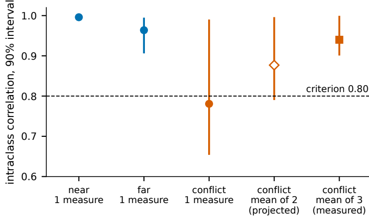
Figure 5: Repeatability of the response in the main study, with 90% bootstrap intervals over histories. The single conflict measurement missed the criterion. The value for the mean of two repeats is a projection; the value for three repeats was measured afterwards.
