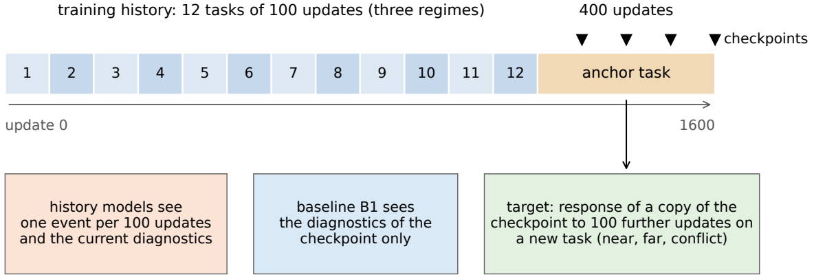
Figure 1: Design of the main study. A network is trained on 12 tasks and then on a common anchor task. At each of four checkpoints, a copy receives 100 updates on a new task and its loss reduction is recorded. History models see one event per 100 updates of the history together with the diagnostics of the current checkpoint. The baseline sees the diagnostics only.
