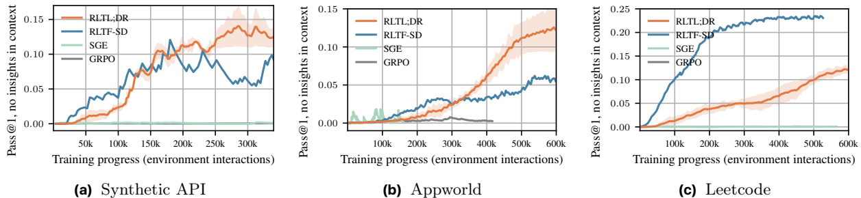
Figure 2 Pass@1 through training, measured only on rollouts without insights (comparable between approaches). Average and std across 3 seeds. GRPO fails to learn since it is starved of learning signal. RLTL;DR and RLTF-SD break through this learning barrier. Leetcode probably overfit.
