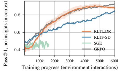
(b) Appworld
