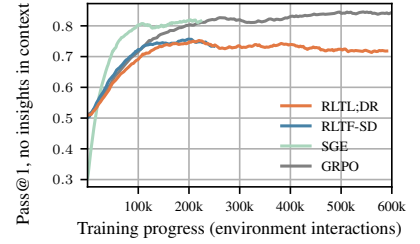
(c) Leetcode
