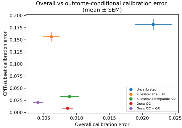
Figure 1: Outcome-conditional (CPIT/subset) vs overall calibration error averaged over all datasets and models for each of the recalibration methods. The vertical and horizontal bars indicate standard error across seeds, datasets and base methods.
