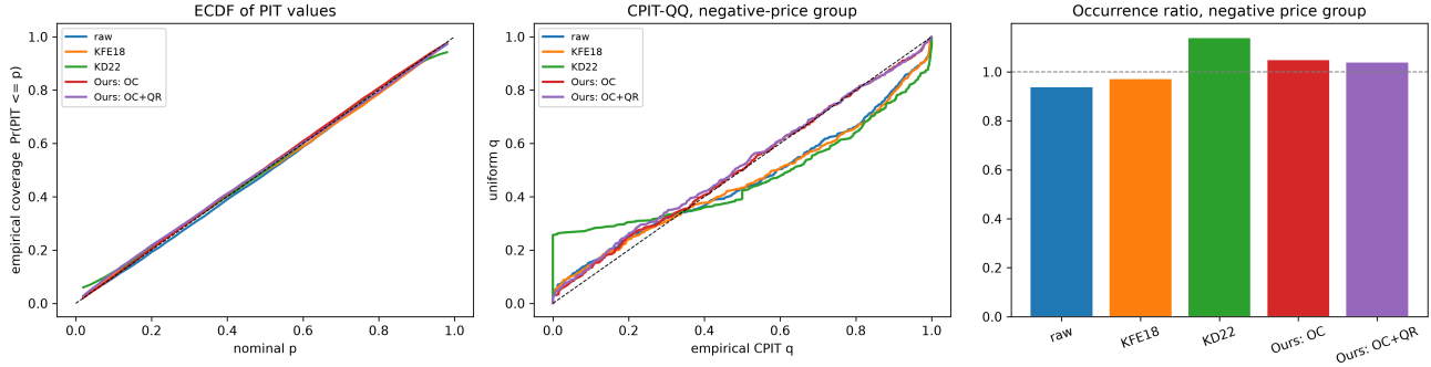
Figure 2: Rolling (182-day) recalibration of the DDNN-JSU, German day-ahead prices, 2019–2020. Left: empirical CDF of PIT values. Middle: quantile-quantile plot of CPIT values for the negative price group against reference values. Right: occurrence ratio of expected over realised events. For the left and middle panels, a calibrated forecast would lie on the 1-1 line, whereas on the right, the occurrence ratio should be close to one.
