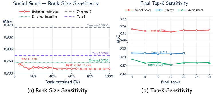
Figure 11: Sensitivity analysis of the retrieval module.
