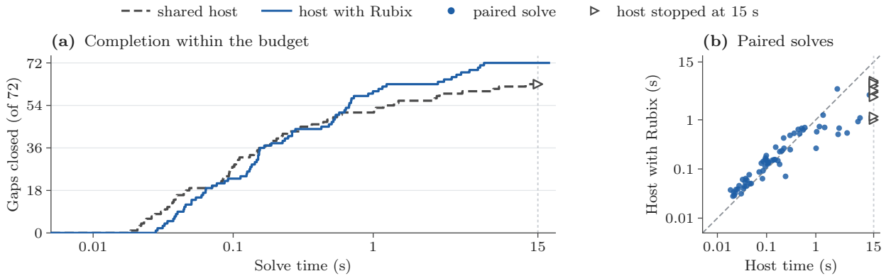
Figure 11: Rubix closes every spatial-alignment gap. Complete SE(3) alignment with a 15s limit and mean-squared gap target 10^{-5} . (a) Solved scenes against time. (b) Paired times; points below the diagonal favor Rubix, and triangles mark nine host timeouts whose completion times are unknown. Both variants return identical poses and matchings throughout; total CPU time includes initialization, assignments, bounds and feasible updates.
