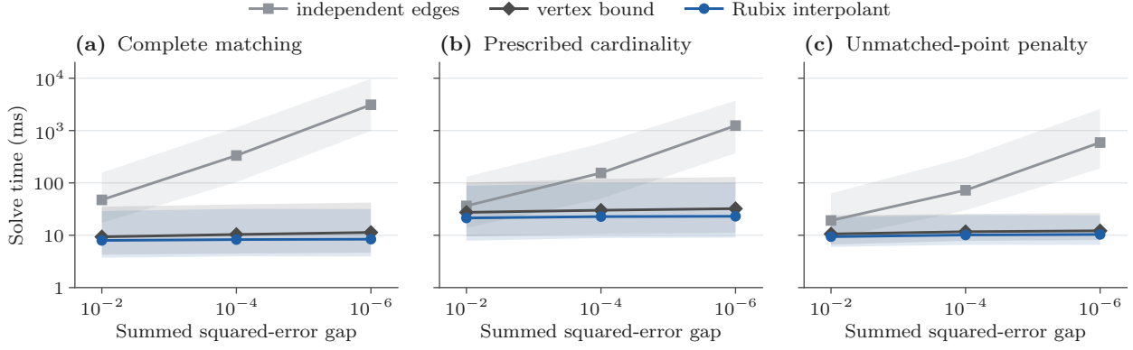
Figure 9: Faster yaw search under three matching models. Median times and interquartile ranges over 72 scenes, including unresolved runs: (a) complete matching after centering; (b) prescribed-cardinality and (c) penalized matching at fixed translation. Rubix and the vertex bound close every gap. From coarse to fine targets, the independent-edge bound closes 72, 72, 50 gaps in (a), 72, 72, 67 in (b), and all 72 in (c). At 10^{-6} , paired median vertex/Rubix time ratios are 1.38, 1.35, 1.21.
