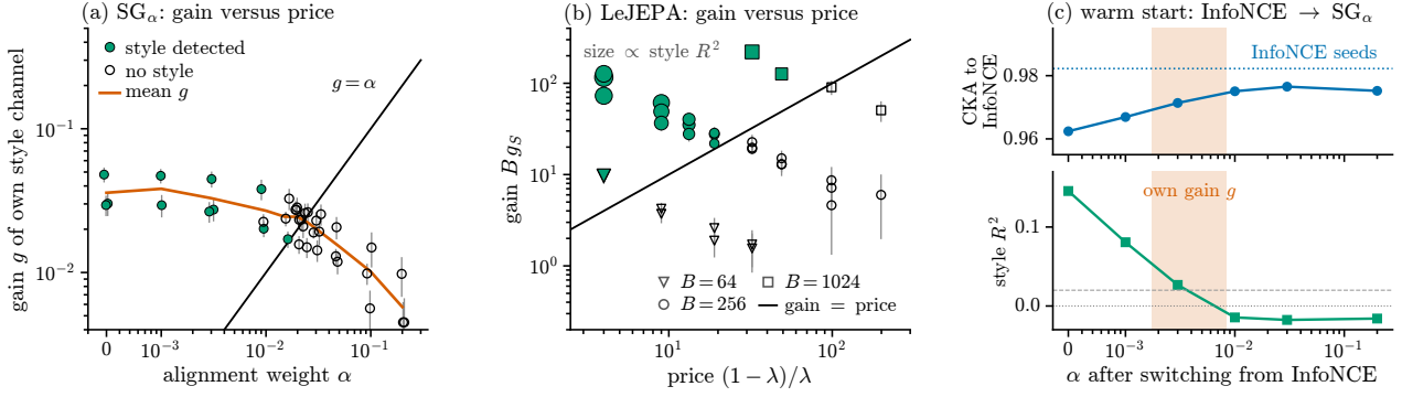
Figure 3 | Gain against price in trained encoders (content–style model, d = 8 ; filled: style detected). (a) SG α : style is detected only when the own-channel gain exceeds \alpha . (b) LeJEPa, three batch sizes: style is detected exactly when Bg_S exceeds the price (1 - \lambda)/\lambda . (c) Warm starts stay close to InfoNCE; the style added by pure SG vanishes once \alpha exceeds their gains (shaded; dashed: detection threshold).
