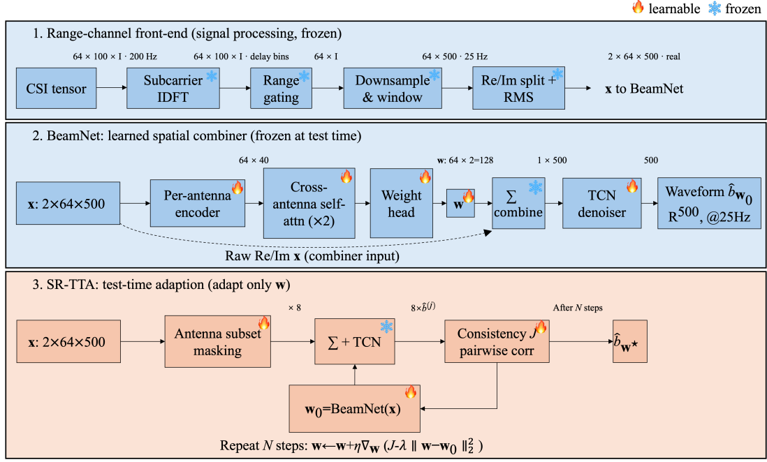
Fig. 2. Proposed pipeline. (1) A frozen front-end reduces the raw CSI to the per-antenna range-channel \mathbf{x} \in \mathbb{R}^{2 \times M \times T} . (2) BeamNet emits M complex combiner weights ( 2M reals) via per-antenna encoding and cross-antenna self-attention, and the combined trace is denoised by a temporal convolutional network (TCN) into the breathing waveform (trained on ground truth, frozen at test time). (3) SR-TTA adapts only the 2M weights per recording, label-free, by maximizing agreement across random antenna subsets.
