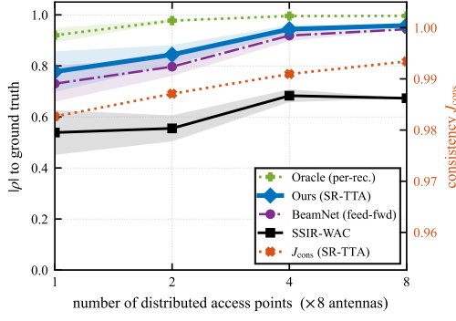
Fig. 5. Scaling under in-band interference: |\rho| vs. number of distributed APs (eight antennas each, \pm SEM over AP subsets), with the oracle ceiling and (right axis) SR-TTA’s achieved consistency J_{\text{cons}} . SSIR-WAC plateaus; SR-TTA scales.
