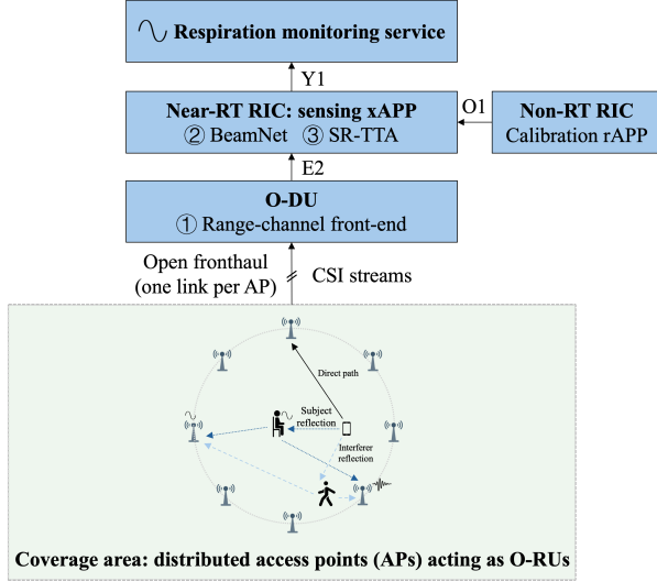
Fig. 1. Considered scenario and proposed O-RAN embedding. Bottom : eight distributed APs surround a seated subject, and a second moving body adds an in-band interferer. Top : the pipeline mapped onto O-RAN, with range-gating (1) at the O-DU, BeamNet (2) and SR-TTA (3) as a near-RT RIC xApp, and one-time calibration as a non-RT rApp feeding the exposed respiration service.
