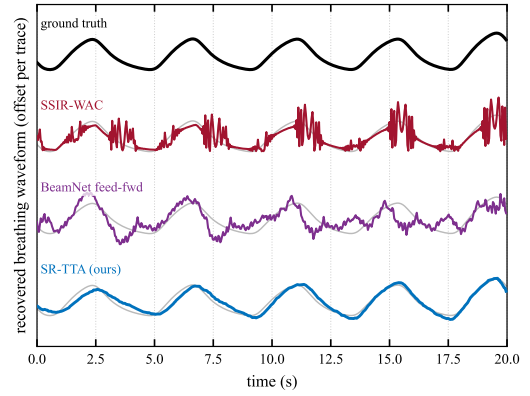
Fig. 4. The in-band recording where adaptation helps most (20 s, estimates offset over the ground truth): SSIR-WAC rides the interferer’s bursts, the feed-forward beam drifts off breathing, and SR-TTA re-locks onto the true rhythm label-free (traces sign-aligned, unit-normalized).
