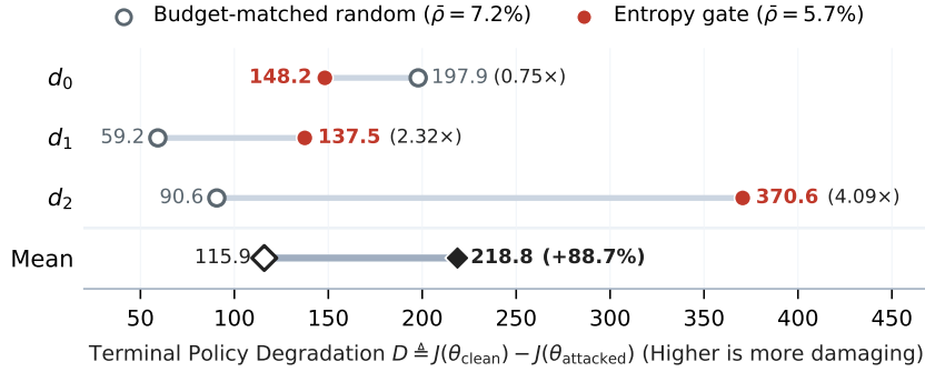
Figure 6: Timing ablation under matched budgets (LunarLander \times FedPG-BR). Fixing all HOW parameters, entropy gating achieves 1.89 \times higher mean degradation than budget-matched random selection across evaluated dynamics.
