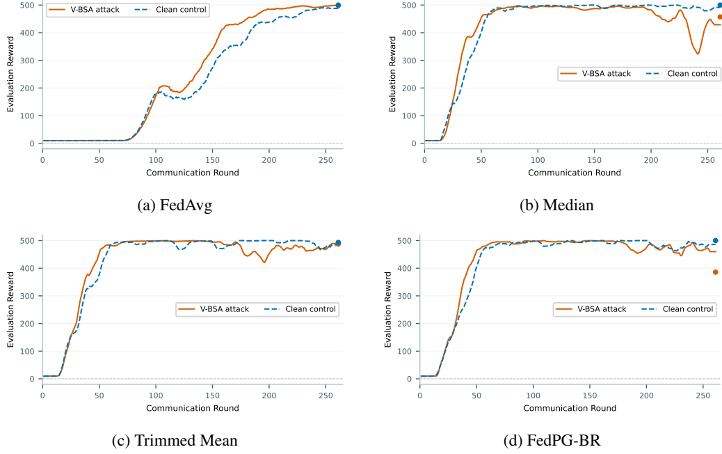
Figure 10: Non-ensemble paradigm on CartPole ( N = 30, M = 10 ). Evaluation trajectories across aggregation rules. Solid curves: V-BSA attack; dashed curves: clean control.
