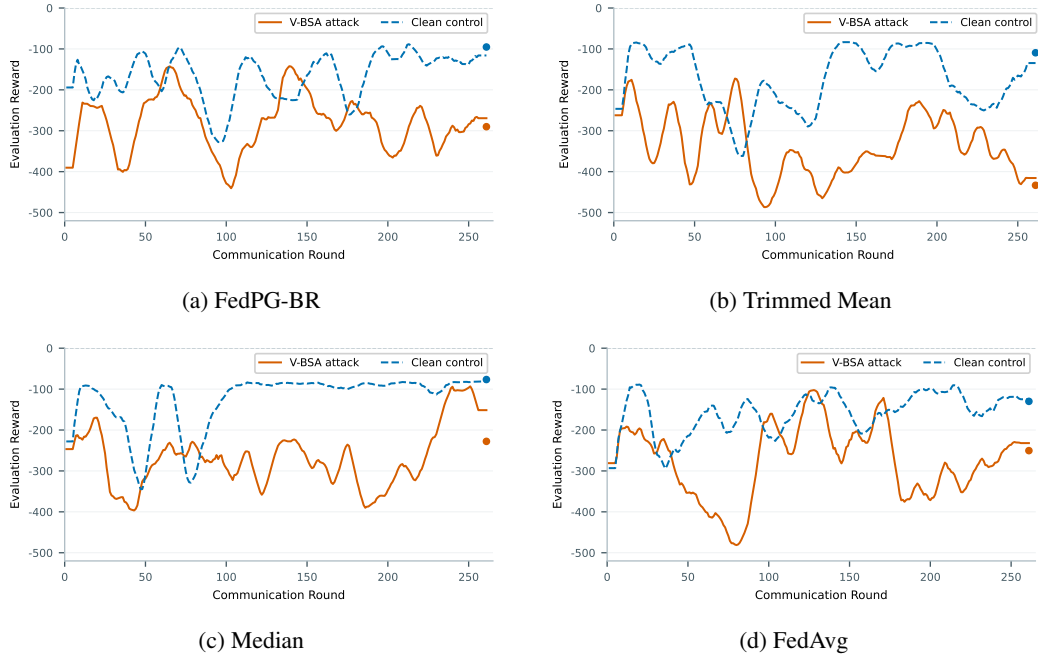
Figure 9: Ensemble paradigm on Acrobot ( K = 5, M = 10 ). Evaluation trajectories across aggregation rules. Solid curves: V-BSA attack; dashed curves: clean control.
