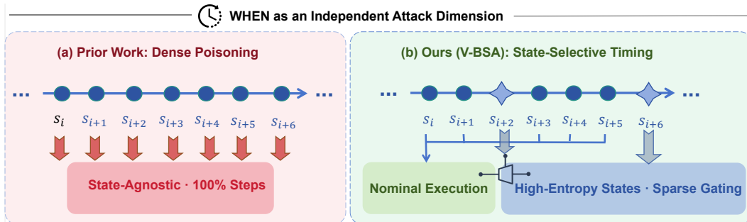
Figure 1: Conceptual comparison of intervention timing in FRL poisoning. (a) Prior work leaves trajectory-level intervention timing implicit, effectively defaulting to dense, state-agnostic intervention across rollout steps. (b) Ours (V-BSA) treats WHEN as an explicit attack dimension: compromised agents maintain nominal execution on routine states and selectively intervene at states identified by policy-entropy gating.
