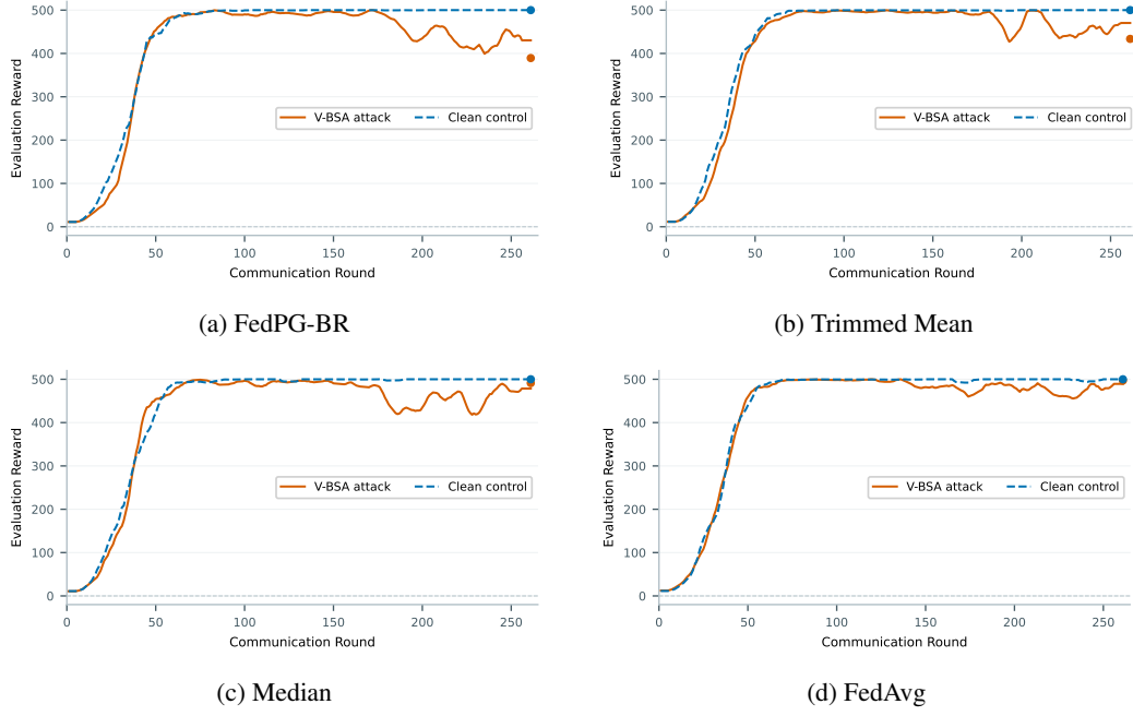
Figure 8: Ensemble paradigm on CartPole ( K = 5, M = 10 ). Evaluation trajectories across aggregation rules. Solid curves: V-BSA attack; dashed curves: clean control.
