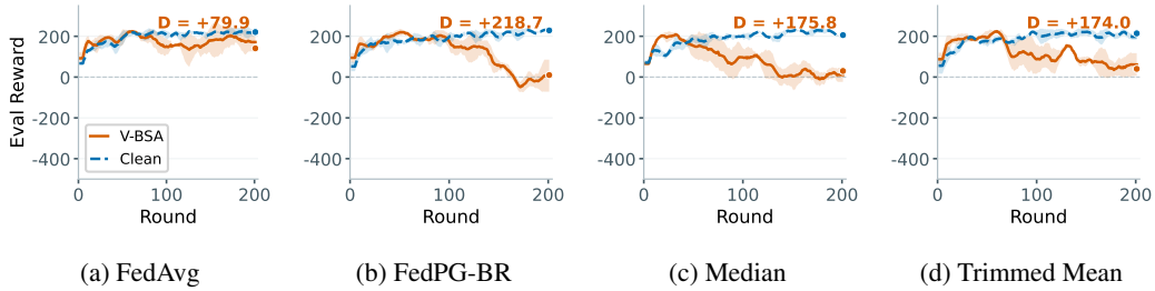
Figure 4: Evaluation dynamics on Ensemble-LunarLander ( K = 5, M = 10 ). Returns of CLEAN vs. V-BSA across four aggregation rules, with shaded bands denoting standard deviation across random seeds.
