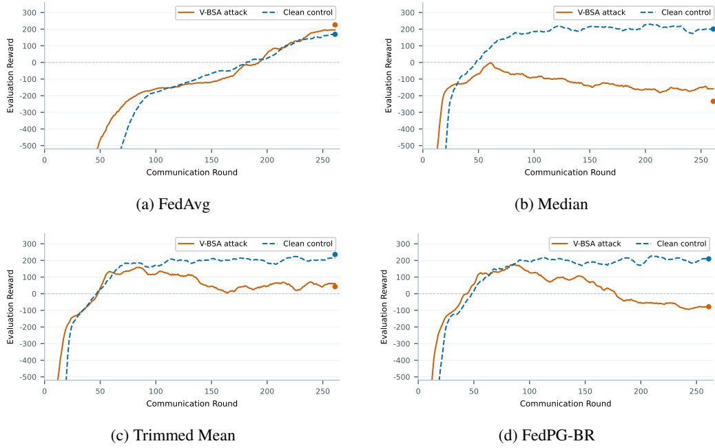
Figure 12: Non-ensemble paradigm on discrete LunarLander-v2 ( N = 30, M = 10 ). Evaluation trajectories across aggregation rules. Solid curves: V-BSA attack; dashed curves: clean control.
