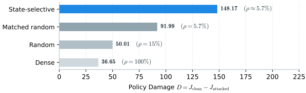
Figure 2: Pilot evaluation of intervention timing. Terminal degradation D on LunarLander under FedPG-BR with fixed update construction across schedules ( \rho ). Entropy gating induces substantially higher degradation than dense and budget-matched baselines.
