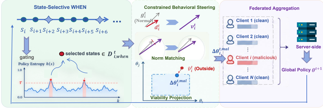
Figure 3: Overview of V-BSA. The attack factorizes into trajectory-level WHEN selection and parameter-space HOW construction: an entropy gate selects sensitive states \mathcal{D}_{i,when}^t , from which a targeted update is synthesized, norm-matched, and constrained by the local empirical envelope B_i^t before server-side aggregation.
