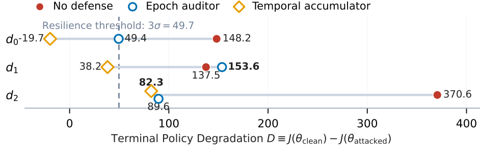
Figure 7: Temporal countermeasures against V-BSA on LunarLander. Terminal degradation D across dynamics d_0, d_1, d_2 under no defense, the epoch auditor, and the temporal accumulator. The dashed line marks the preregistered resilience threshold ( 3\sigma = 49.7 ).
