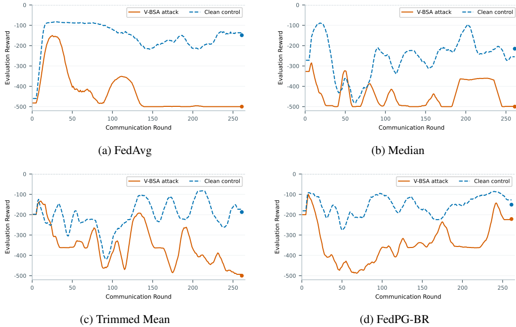
Figure 11: Non-ensemble paradigm on Acrobot ( N = 30, M = 10 ). Evaluation trajectories across aggregation rules. Solid curves: V-BSA attack; dashed curves: clean control.
