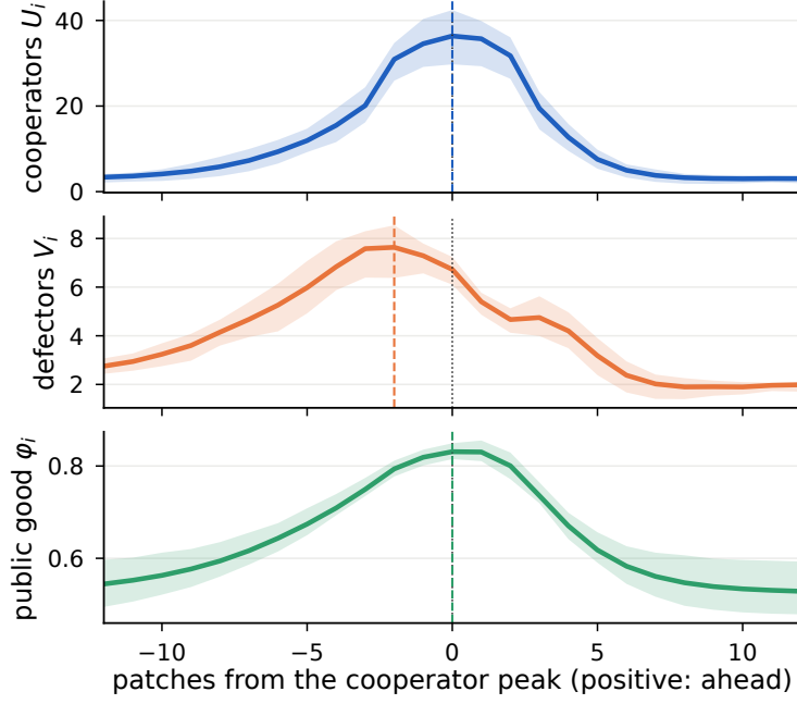
Figure 11: Aligned profiles of the traveling bands. For each of the 50 coherently traveling runs and each snapshot t = 200, \dots, 400 , the profiles are shifted so that the maximum of the cooperator profile, smoothed over five patches, is at 0. They are reflected so that the band travels to the right and are then averaged over snapshots. Lines show the mean over runs and shading the interquartile range over runs. Dashed lines mark the maximum of each mean profile, and the horizontal axis is in patches. The defector maximum lies two patches behind the cooperator maximum.
